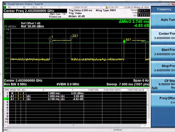
NTVN-3DH5-Ant1-2402
