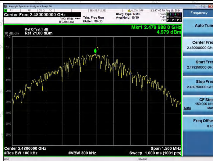
DH5-Ant1-2480-0~Reference-PASS
