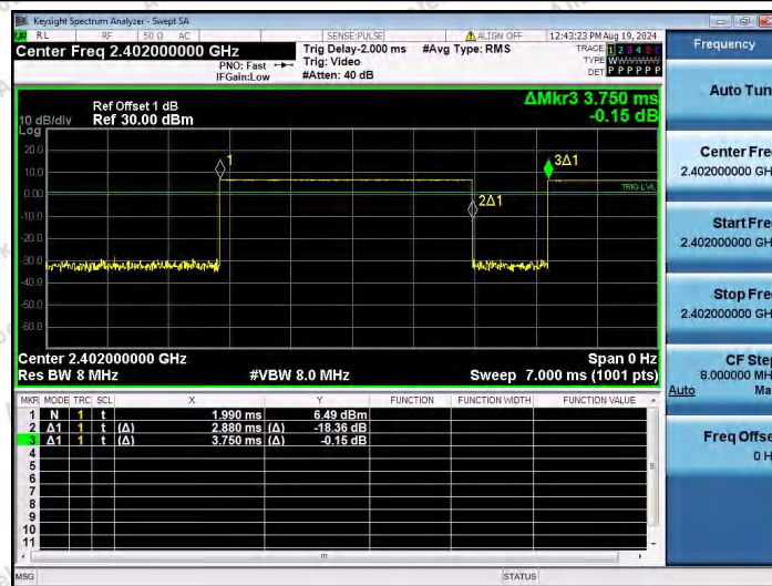
NTNV-DH5-Ant1-2402
