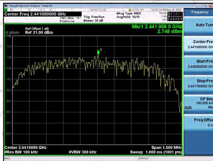
2DH5-Ant1-2441-0~Reference-PASS
