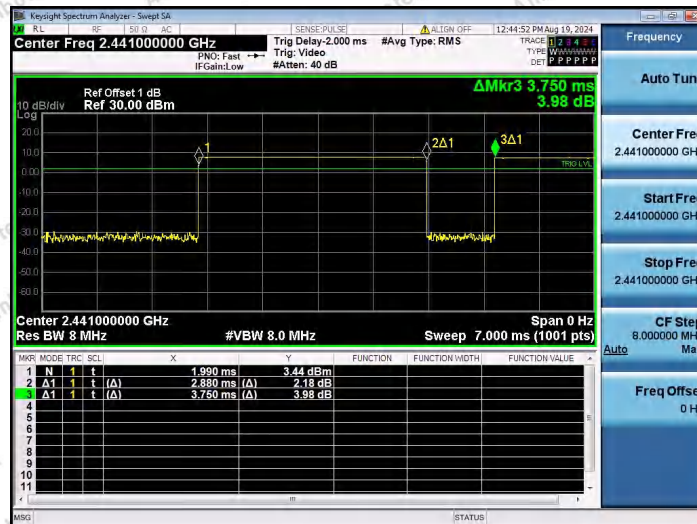
NTNV-DH5-Ant1-2441
