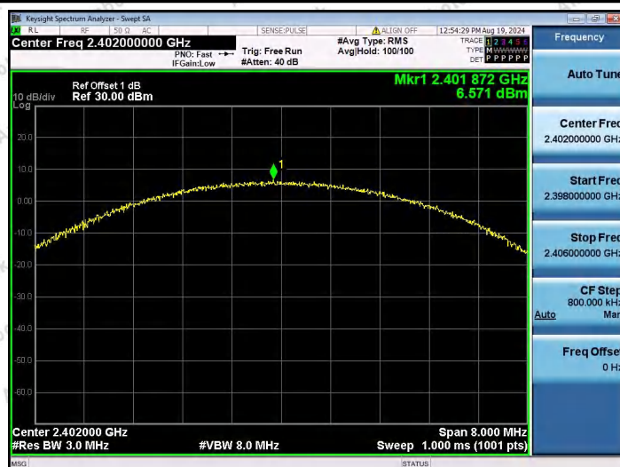
3DH5-Ant1-2402-PASS
