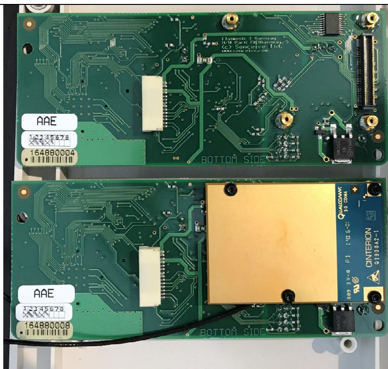
Underside of main PCB – shown with and without 3G module
