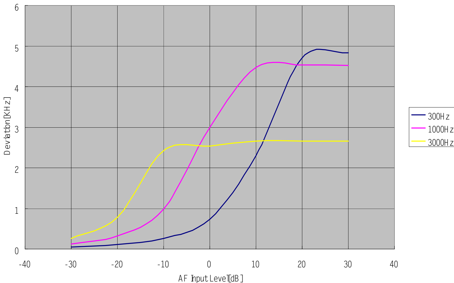
Modulation Limiting / 134.125MHz / 25KHz Mode
