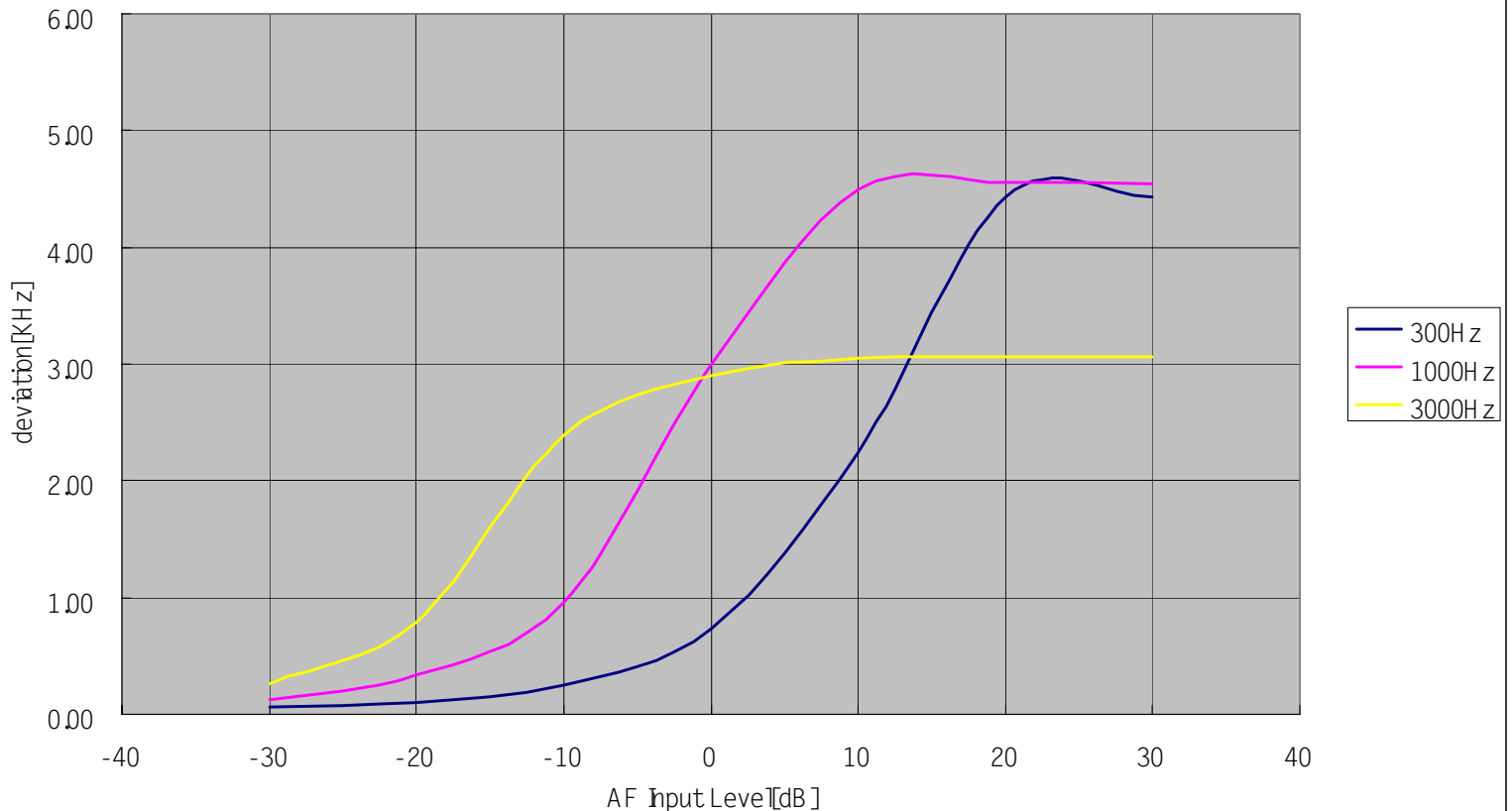
Modulation Limiting / 173.975MHz / 15KHz Mode
