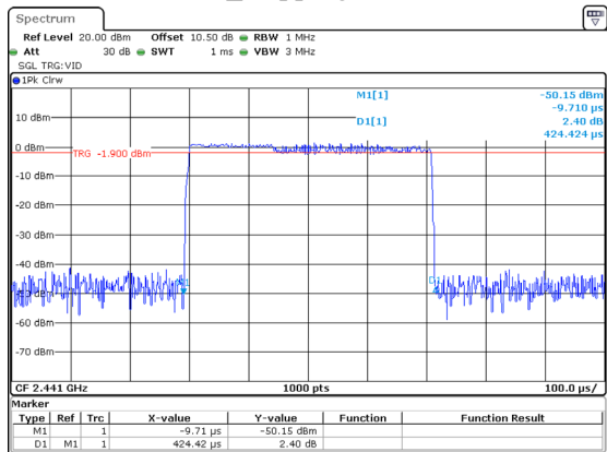
2DH1_Hopping 0.424ms
