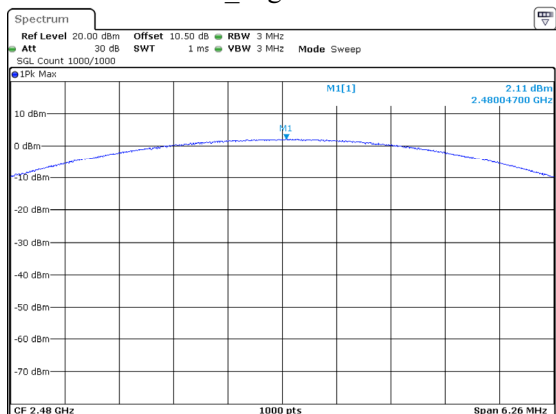
2DH1_High 2.11dBm
