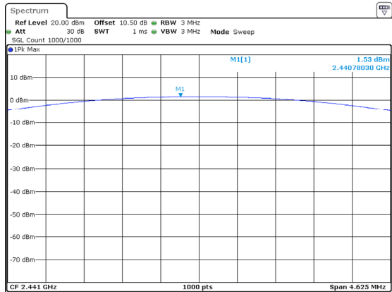
DH1_Middle 1.53dBm
