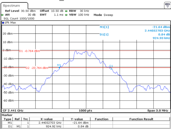
DH1_Middle 0.925MHz
