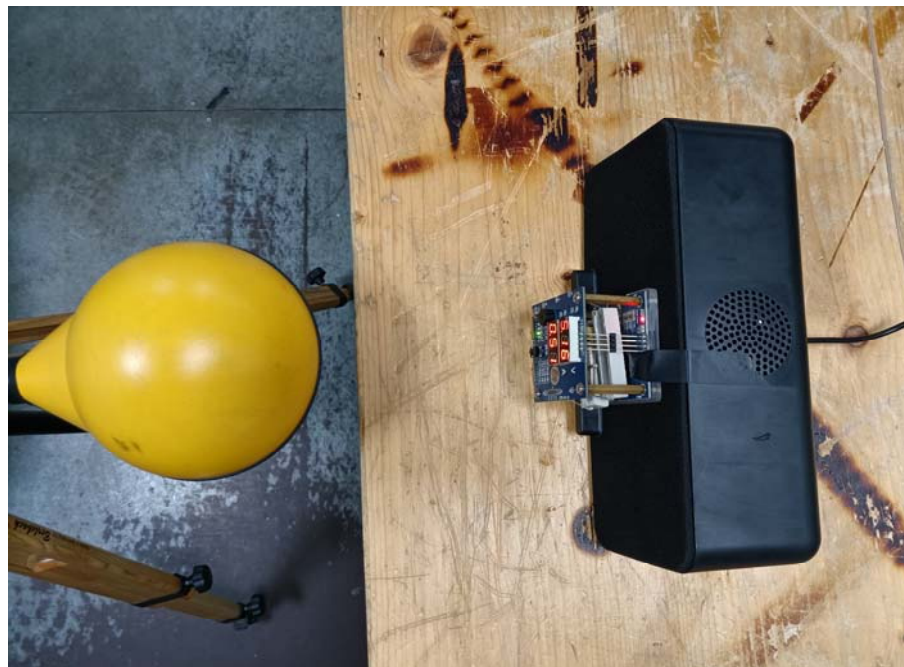
H-Field Strength View Position A (Distance 15cm)
