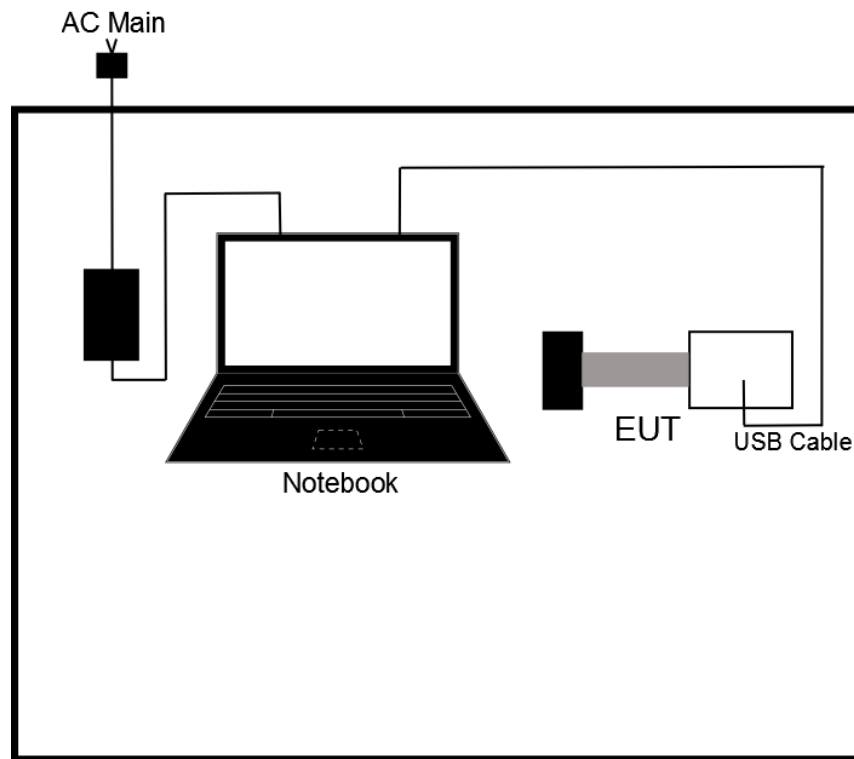
Test Setup Diagram - Radiated Test_ Above 1GHz
