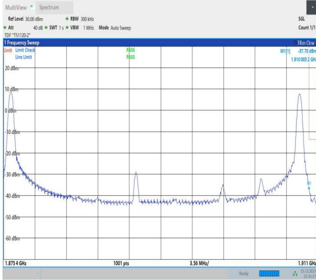
15MHz-20MHz_64QAM@64QAM-64QAM_18929-19100_1RB#0@75RB#0-1RB#99@100RB#0
