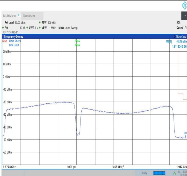
15MHz-20MHz_64QAM@64QAM-64QAM_18929-19100_1RB#0@75RB#0-1RB#99@100RB#0
