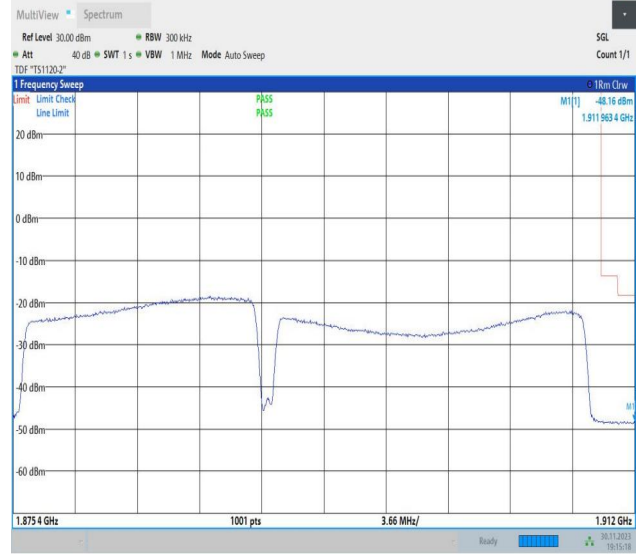
15MHz-20MHz_QPSK@QPSK-QPSK@QPSK_18929-19100_75RB#0@75RB#0-100RB#0@100RB#0
