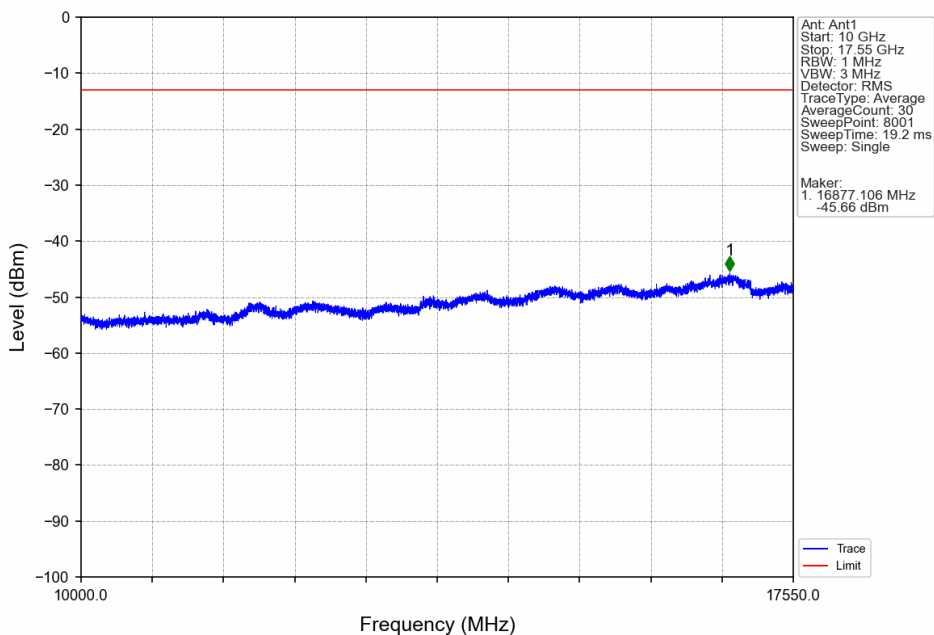
Band4 3MHz 16QAM HCH 1753.5MHz RB 1 0 NTV
