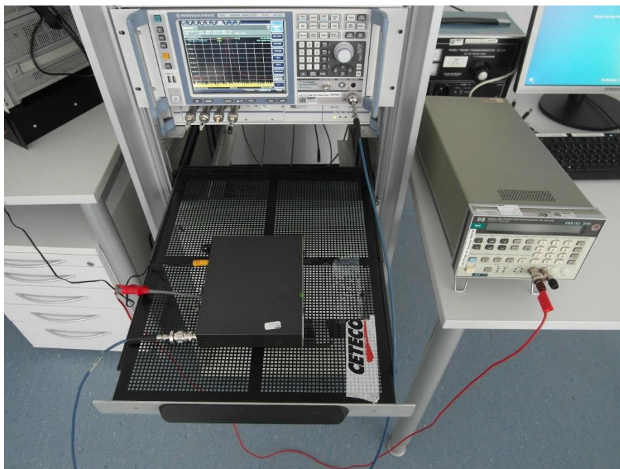
Photo 11: spectrum analyzer
