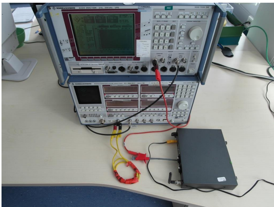
Photo 10: audio analyzer
