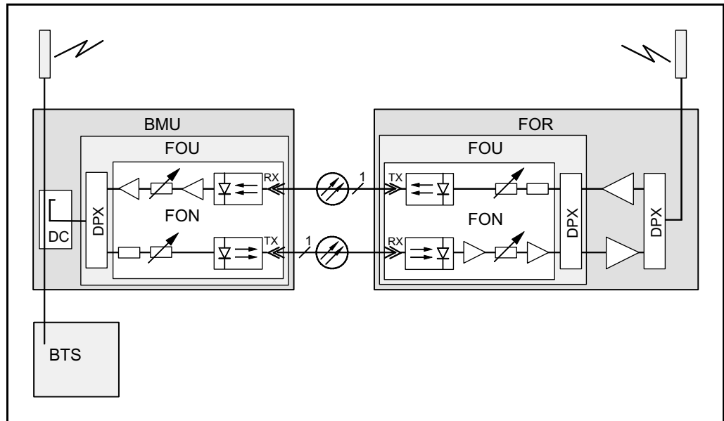
Figure 4-8. FOU inserted in the BMU and FOR
