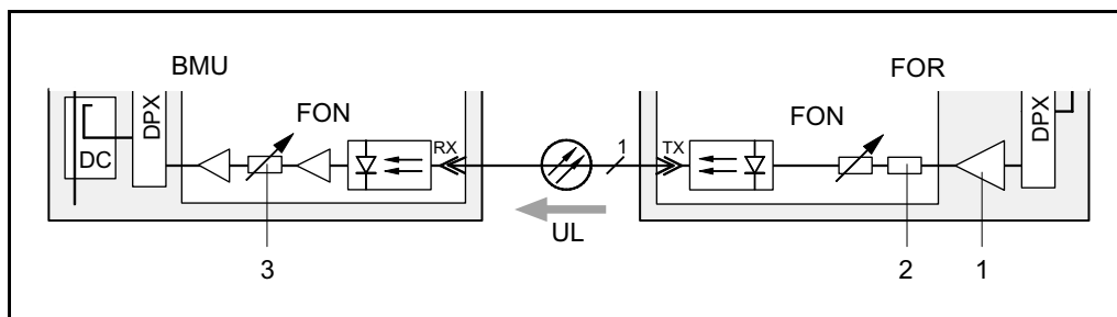
Figure 4-5. Uplink RF transmission path
