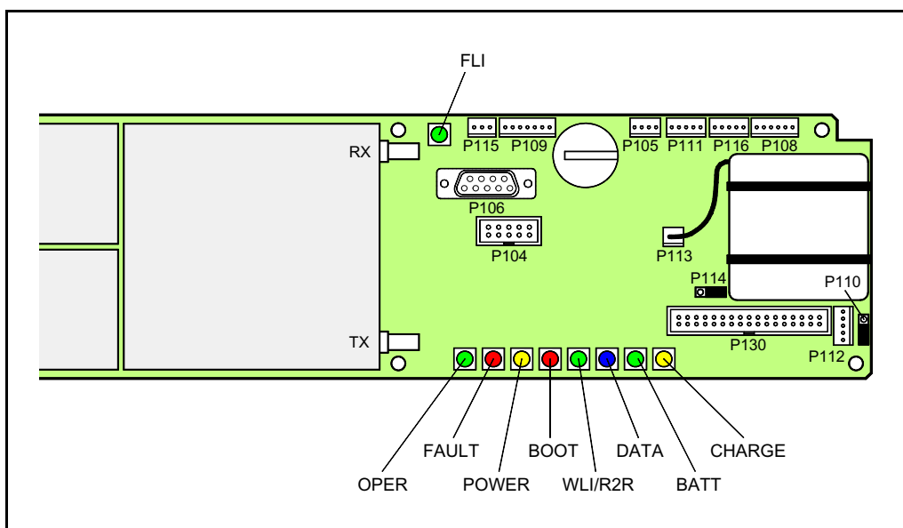
Figure 3-5. FON indicators and ports
