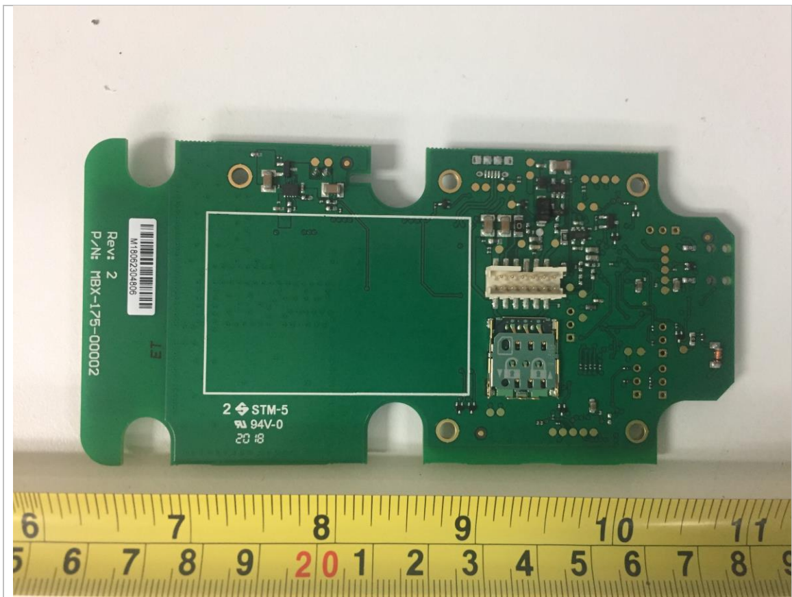
EUT Main PCBA – Bottom
