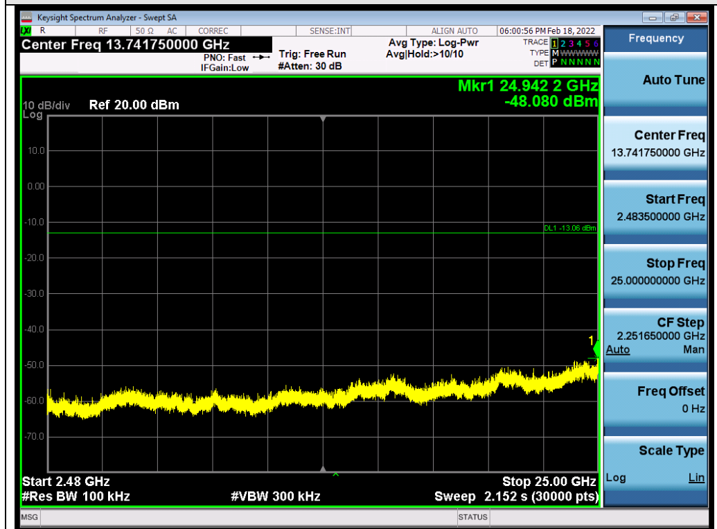
Test_Graph_O-QPSK_ANT1_2440_Higher Band Emissions
