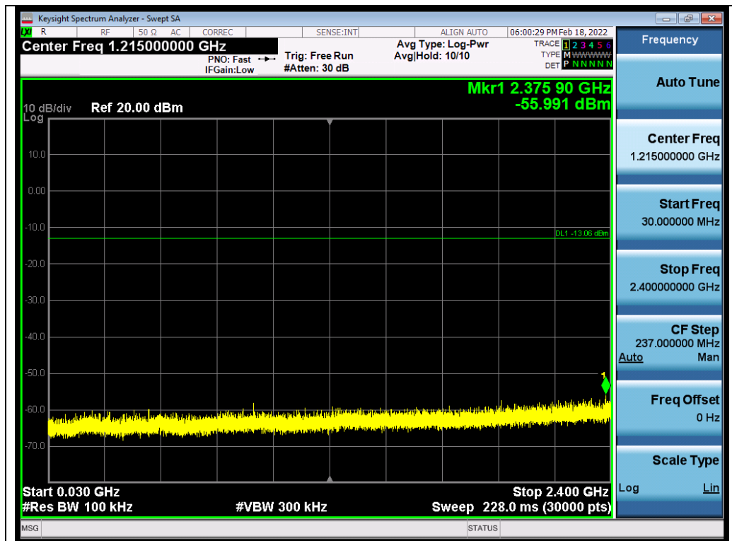
Test_Graph_O-QPSK_ANT1_2440_Lower Band Emissions
