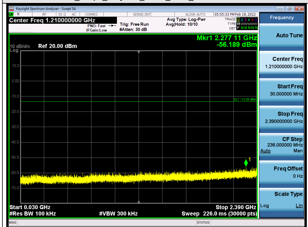
Test_Graph_O-QPSK_ANT1_2405_Lower Band Emissions
