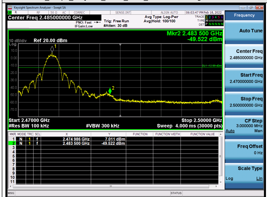
Test_Graph_O-QPSK_ANT1_2475_Higher Band Edge Emissions
