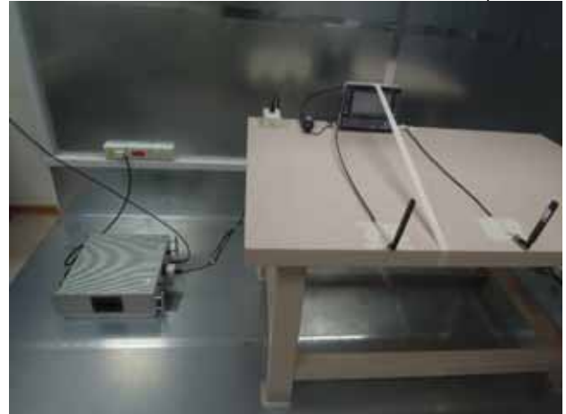
FCC_15_407_Conduction_VM3AC2235G00006_Setup
