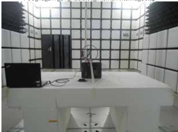
FCC_15_247_BT_Radiated_Internal Antenna_Setup
