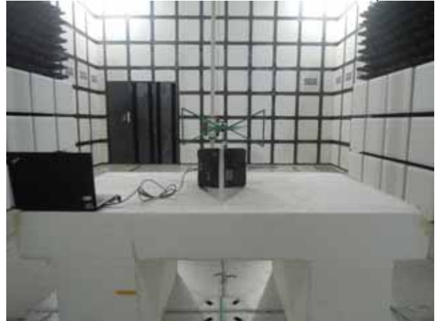
FCC_15_247_BLE_Radiated_External Antenna_Setup
