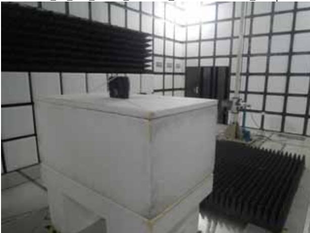
FCC_15_247_WLAN_Radiated_External Antenna_Setup
