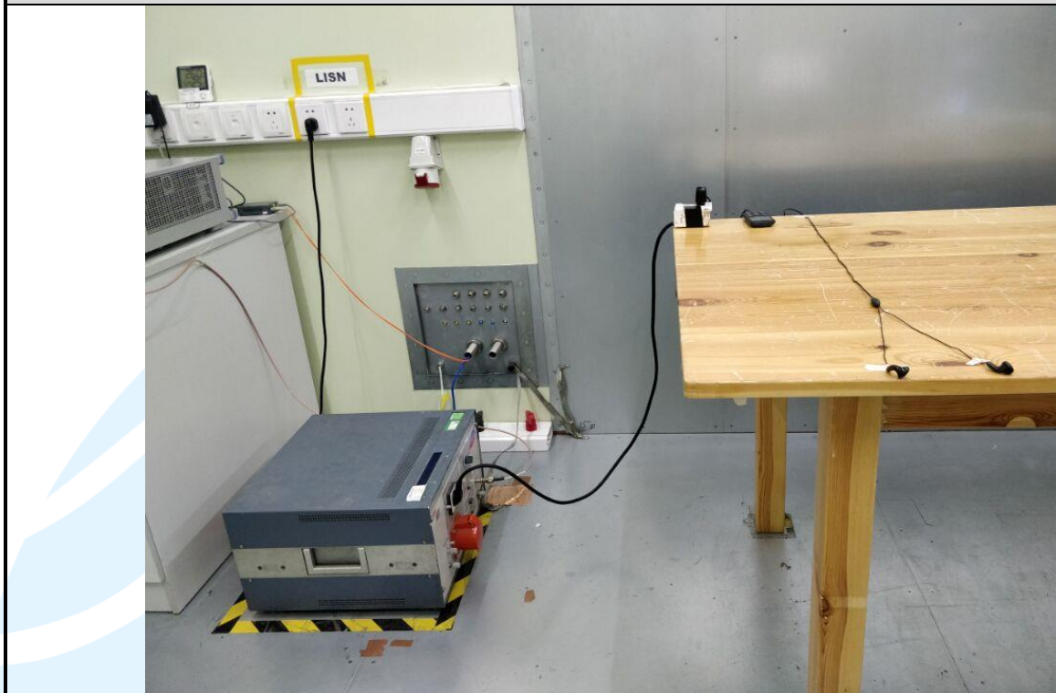
Conducted Emission Test Setup - Mode 3
