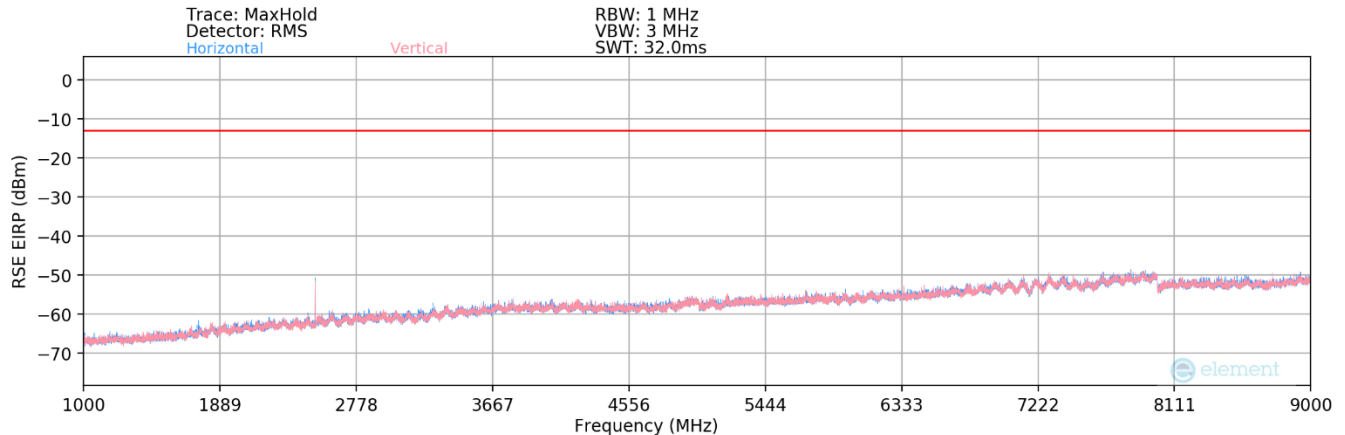
Plot 7-47. Radiated Spurious Plot Above 1GHz (LTE Band 26/5)
