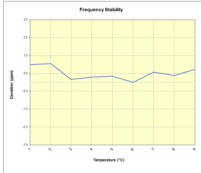
Plot 7-54. LTE Band 26/5 Frequency Stability Chart
