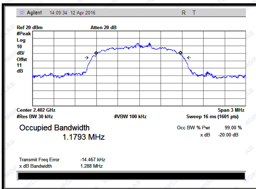
(Plot G: Channel = 2402 @ 8-DPSK)
