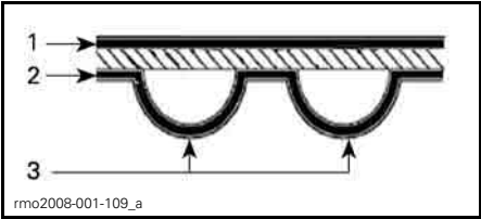
DRIVE BELT SURFACES 1. Outer surface 2. Teeth side surface 3. Tooth
