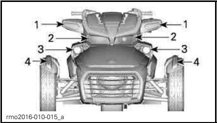
TYPICAL - LIGHTS LOCATION — FRONT OF VEHICLE — F3-T AND F3 LIMITED NORTH AMERICAN MODELS
