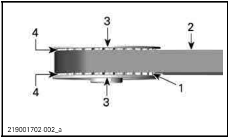
TYPICAL - FRONT SPROCKET 1. Front sprocket teeth 2. Belt 3. Sprocket flange 4. Gap between flange and belt
