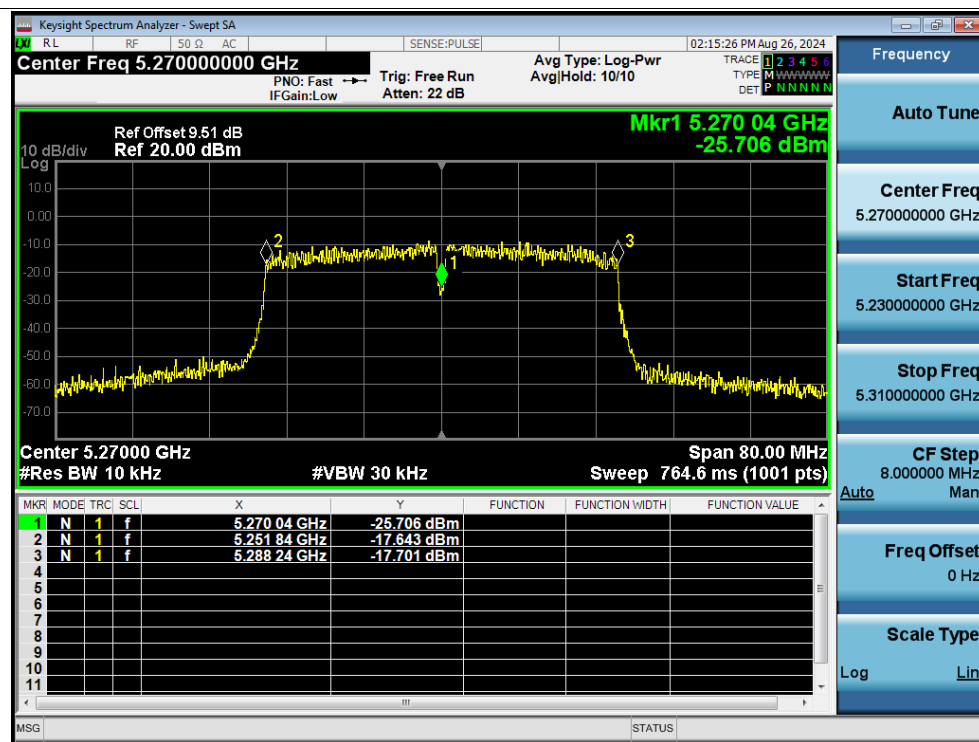
Freq. Stability 30C 3.3V n40 5270MHz Ant1 0 Minutes
