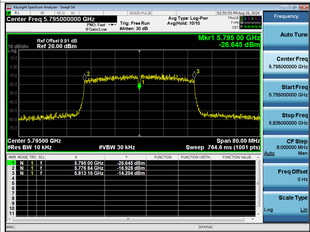
Freq. Stability 50C 3.3V n40 5795MHz Ant1 0 Minutes
