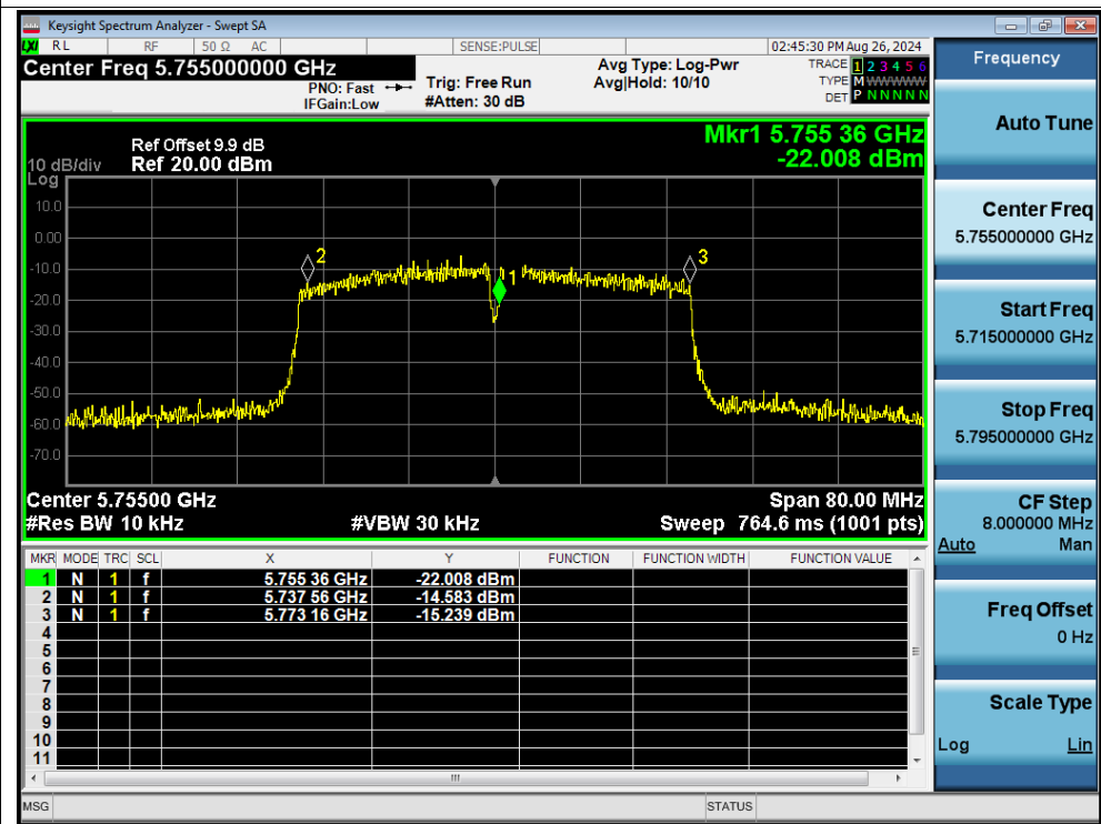
Freq. Stability 30C 3.3V n40 5755MHz Ant1 0 Minutes
