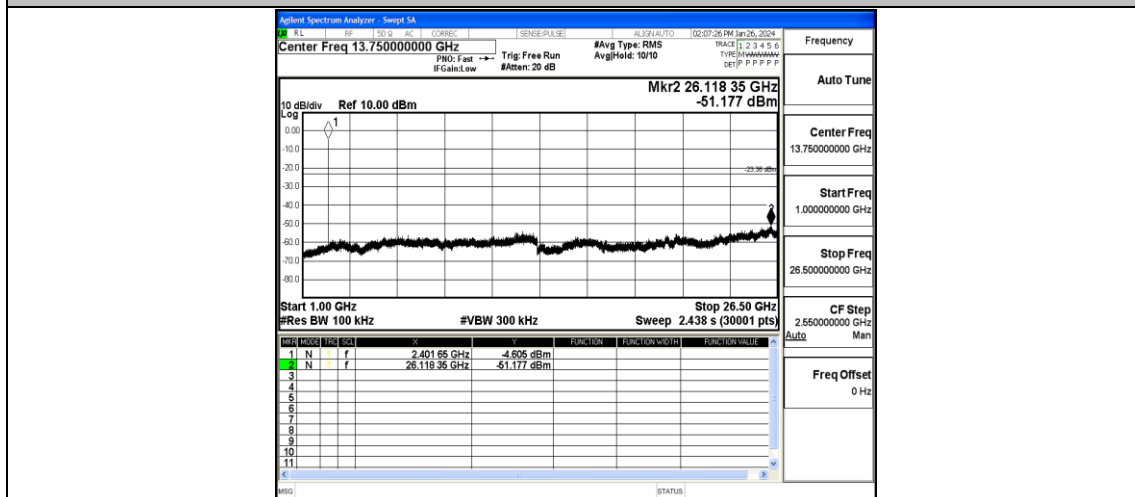
3DH5-Ant1-2402-1000~26500-PASS
