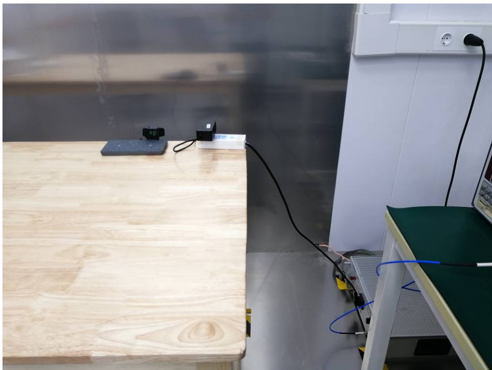
Conducted emission(Watch)
