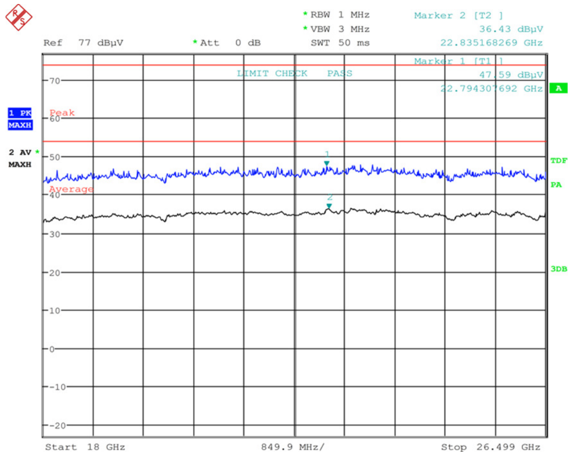
Plot 6-314: Radiated Emissions of Carrier - TC #7 Concrete Container
