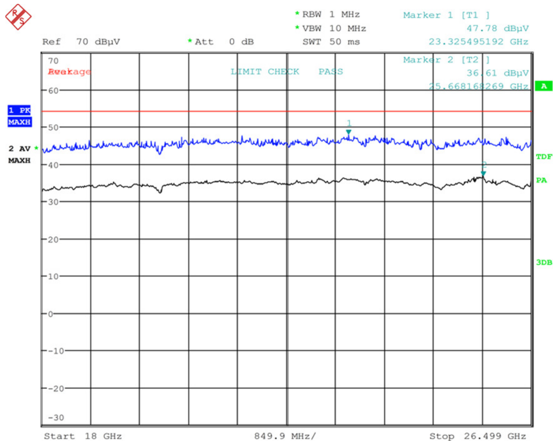
Plot 6-335: Radiated Emissions of Carrier - TC #8 Concrete Container
