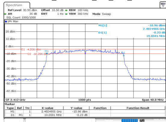
802.11ax20_2412MHz_RU_Full_Chain 0
