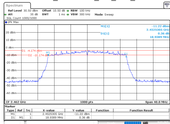
802.11ax20_2462MHz_RU_Full_Chain 0
