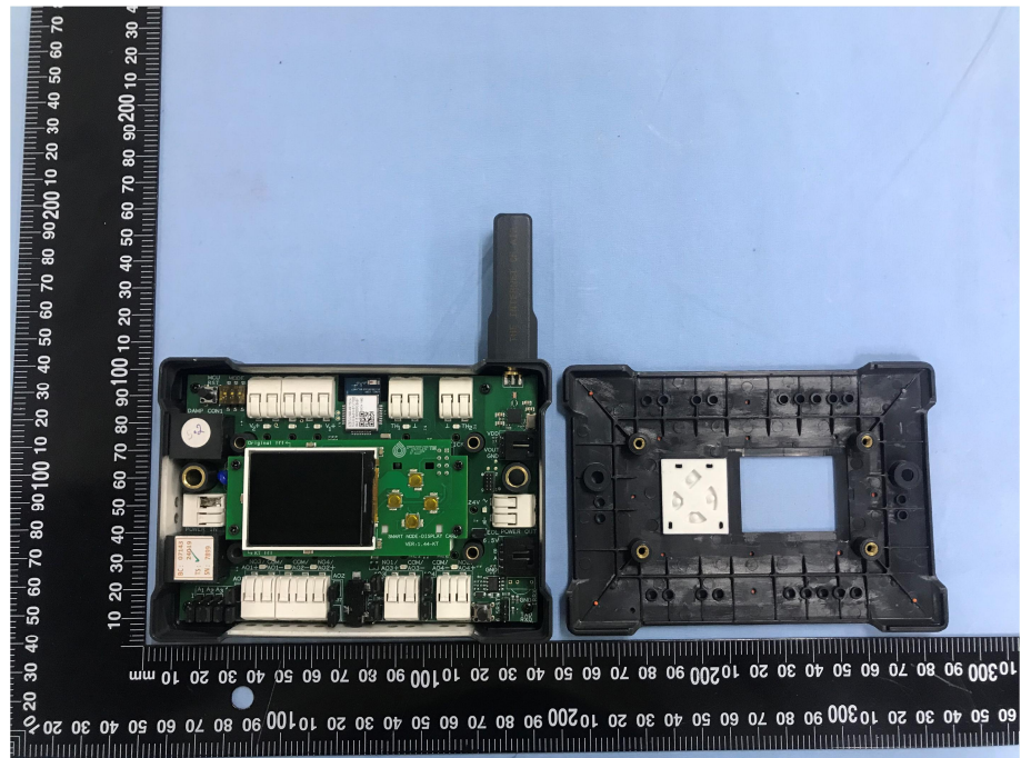
EUT Housing and Board View
