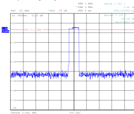
EDR ( \pi/4 -DQPSK): Pulse time, Middle Channel, 2DH1
