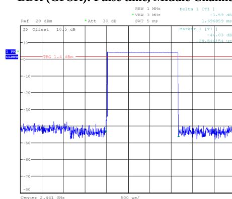
BDR (GFSK): Pulse time, Middle Channel, DH3
