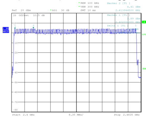
EDR (π/4-DQPSK): Number of Hopping Channels
