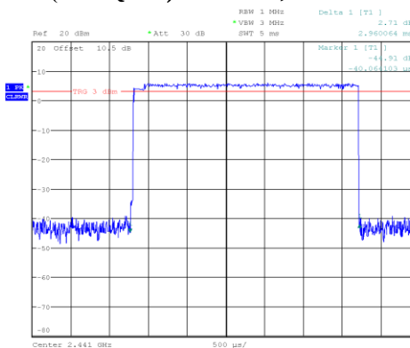
EDR ( \pi/4 -DQPSK): Pulse time, Middle Channel, 2DH5
