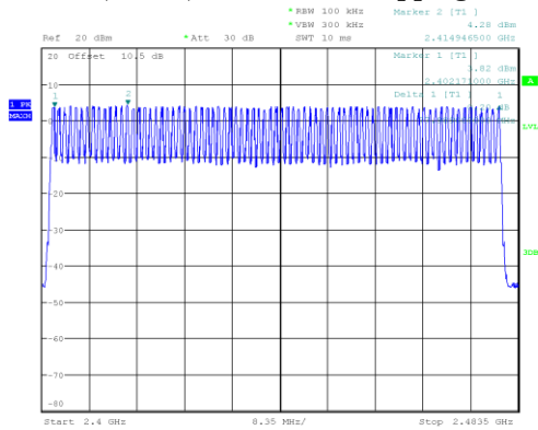
BDR (GFSK):Number of Hopping Channels
