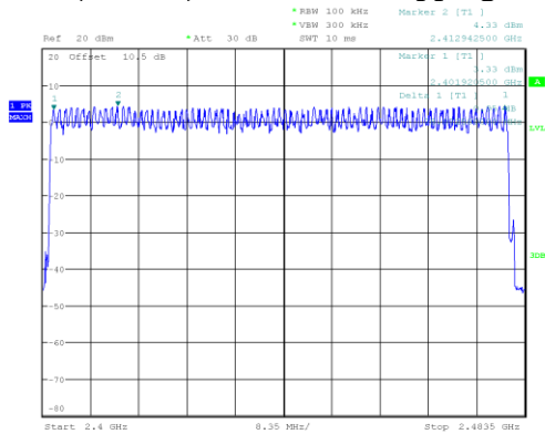
EDR (8DPSK): Number of Hopping Channels
