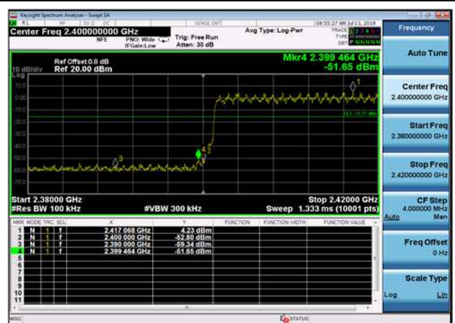
8DPSK,Hopping,3DH5,Band Edge LowRange
