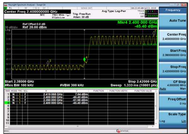
DQPSK,Hopping,2DH5,Band Edge LowRange
