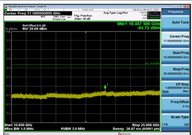
8DPSK,2480MHz,3DH5,Plot 4,10000MHz~25000MHz
