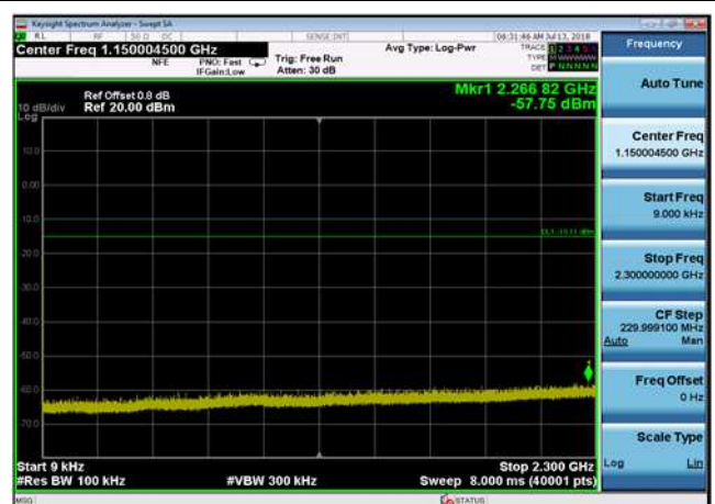
8DPSK,2441MHz,3DH5,Plot 2,0.009MHz~2300MHz
