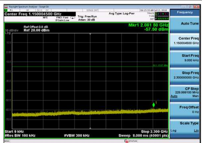
DQPSK,2441MHz,2DH5,Plot 2,0.009MHz~2300MHz
