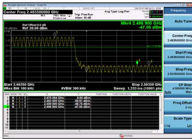
DQPSK,Hopping,2DH5,Band Edge HighRange
