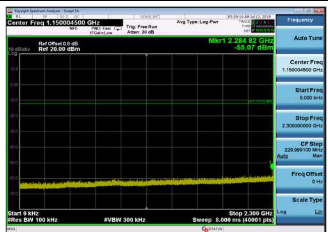
GFSK,2441MHz,DH5,Plot 2,0.009MHz~2300MHz
