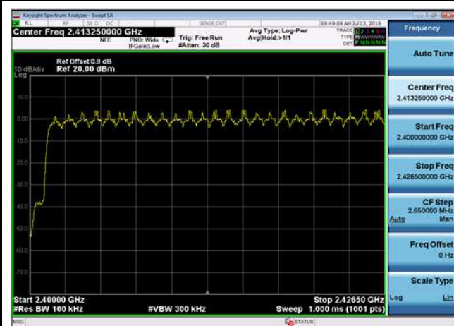
DQPSK,Hopping,2DH5,2400~2426.5MHz
