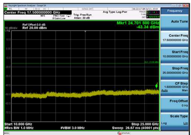
DQPSK,2480MHz,2DH5,Plot 4,10000MHz~25000MHz
