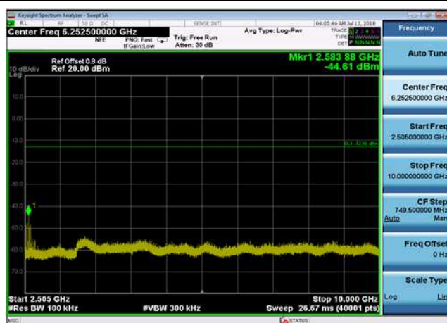
GFSK,2480MHz,DH5,Plot 3,2505MHz~10000MHz
