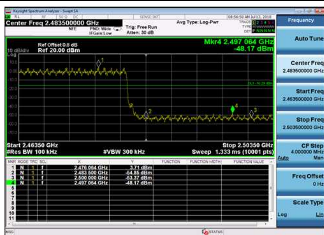
8DPSK,Hopping,3DH5,Band Edge HighRange
