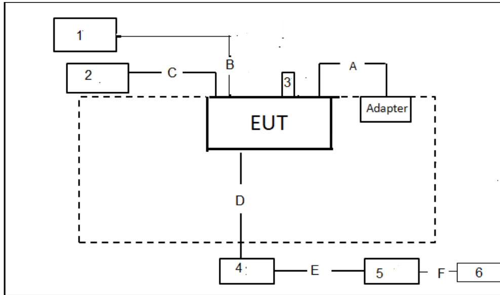
Connection Diagram
