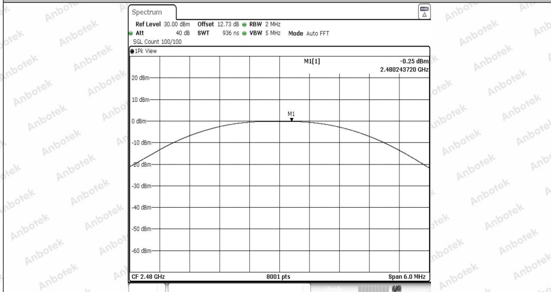
BLE_1M-Ant1-2480-PASS
