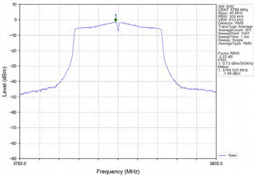
802.11n(HT20)_MCH_5785MHz_Ant2_NTNV
