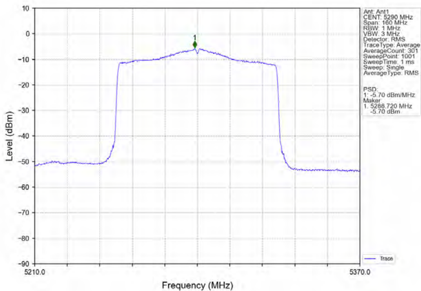
802.11ax(HEW80)_MCH_5290MHz_SU_/_Ant1_NTNV
