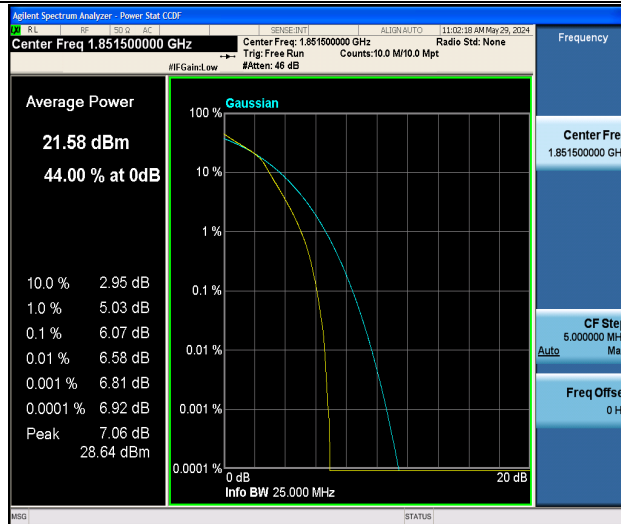
Band2-3MHz-16QAM-18615-15RB#0-PASS
