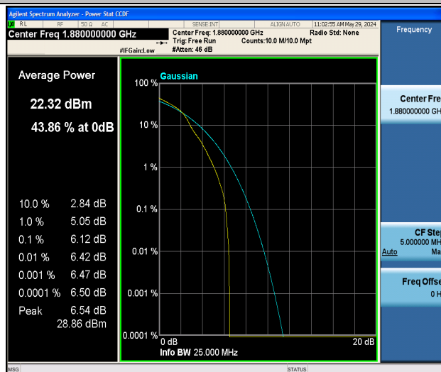
Band2-3MHz-16QAM-18900-1RB#0-PASS
