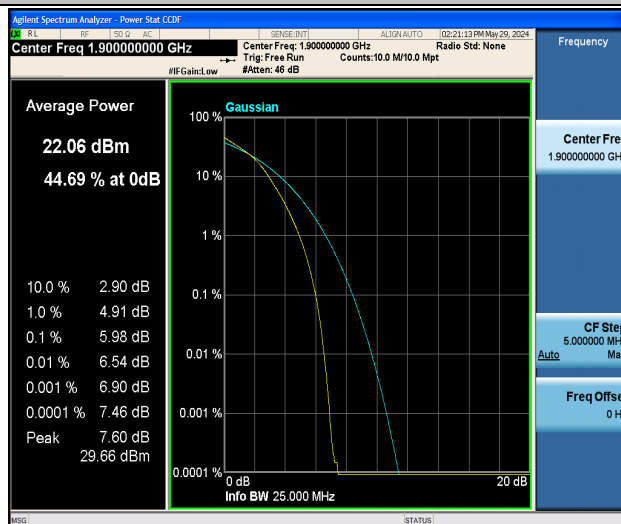
Band2-20MHz-16QAM-19100-100RB#0-PASS
