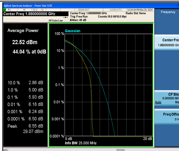
Band2-10MHz-16QAM-18900-1RB#0-PASS
