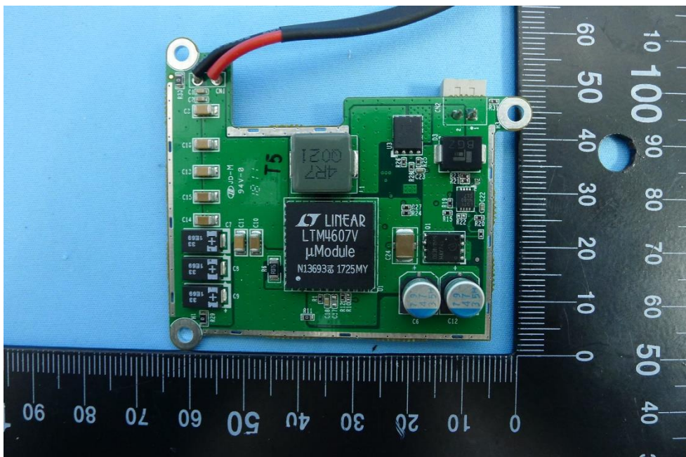
(27) EUT Photo
