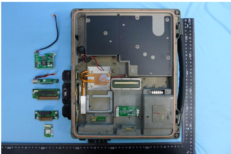
(27) EUT Photo
