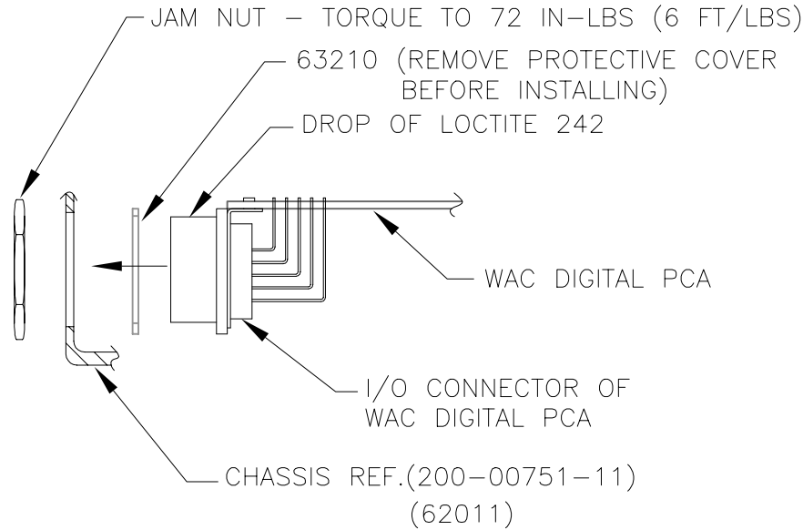
SECTION G-G [7]
