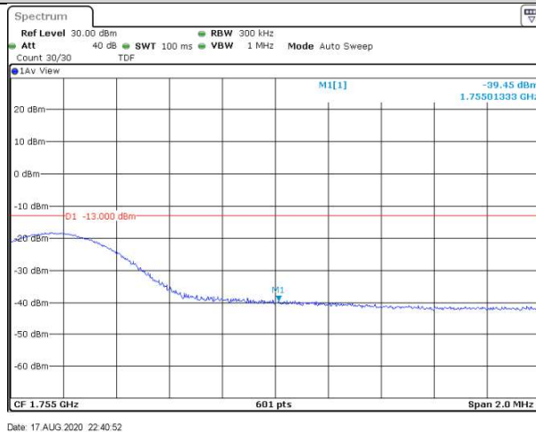
Band4-15MHz-QPSK-20325-1RB#74
