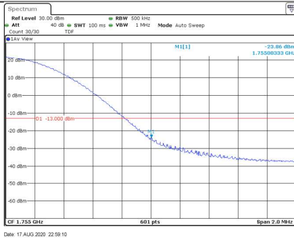
Band4-20MHz-QPSK-20300-1RB#0
