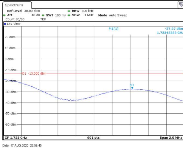
Band4-20MHz-QPSK-20300-100RB#0
