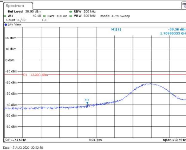
Band4-10MHz-16QAM-20000-1RB#0
