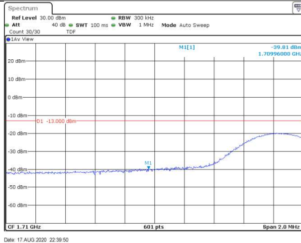
Band4-15MHz-QPSK-20025-75RB#0
