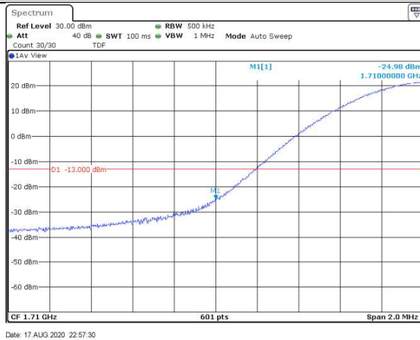
Band4-20MHz-16QAM-20050-1RB#99
