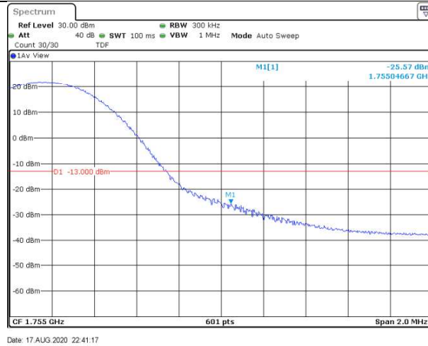
Band4-15MHz-QPSK-20325-75RB#0
