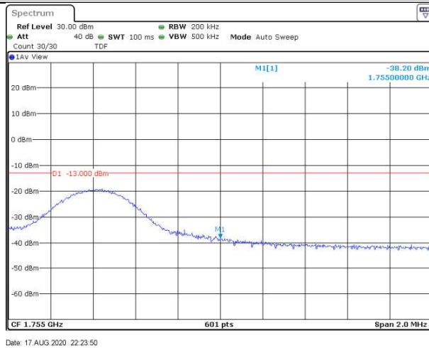
Band4-10MHz-16QAM-20350-1RB#49
