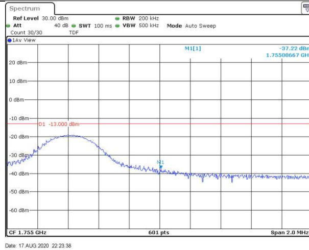
Band4-10MHz-QPSK-20350-50RB#0
