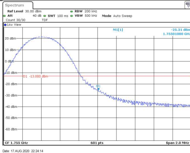
Band4-10MHz-16QAM-20350-50RB#0
