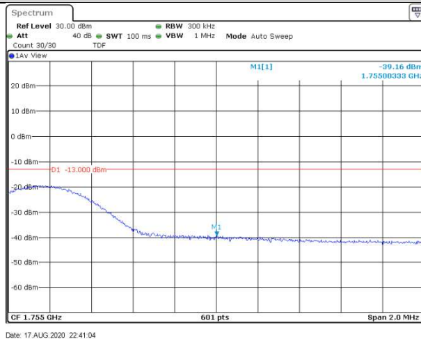
Band4-15MHz-16QAM-20325-1RB#74
