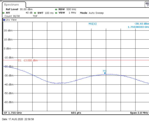
Band4-20MHz-16QAM-20300-1RB#99
