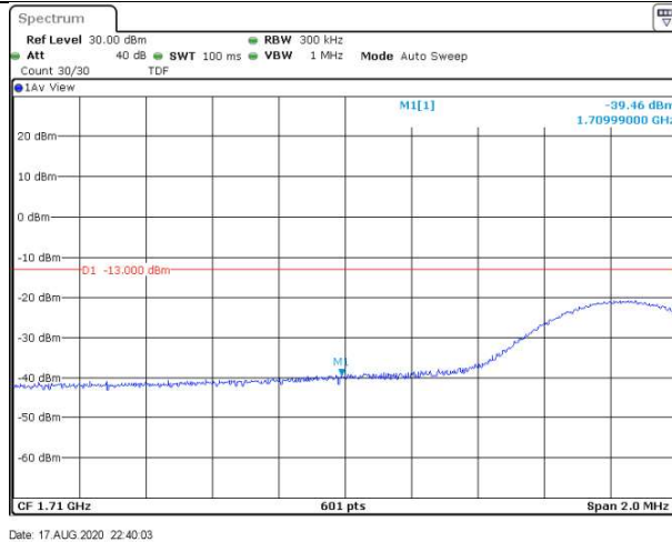
Band4-15MHz-16QAM-20025-75RB#0
