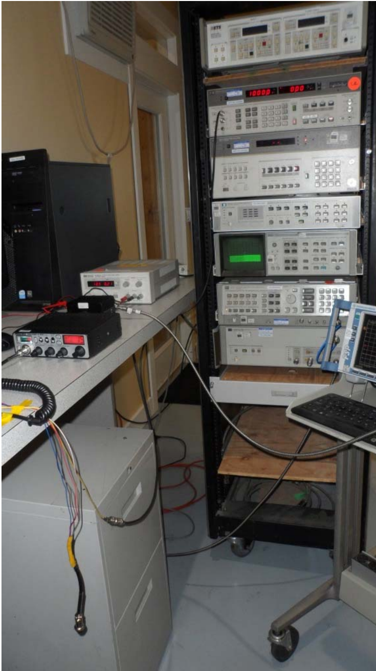
Figure E20.2 – Setup Photo – Audio Response Measurements
