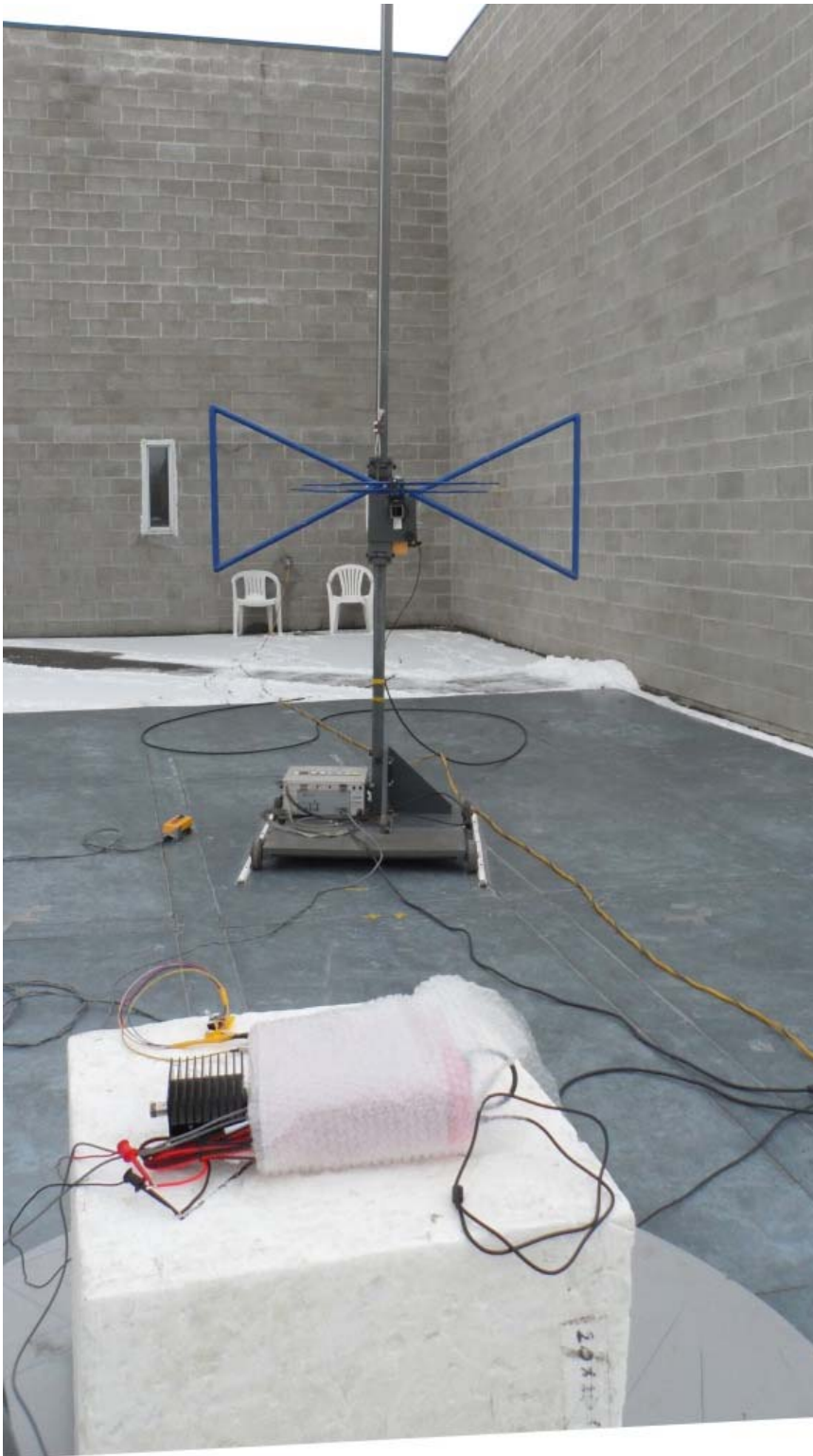
Figure E20.7 – Setup Photo – Radiated Measurements - Horizontal
