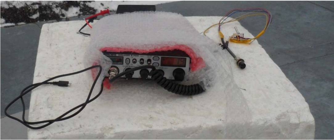
Figure E20.5 – Setup Photo – Radiated Measurements
