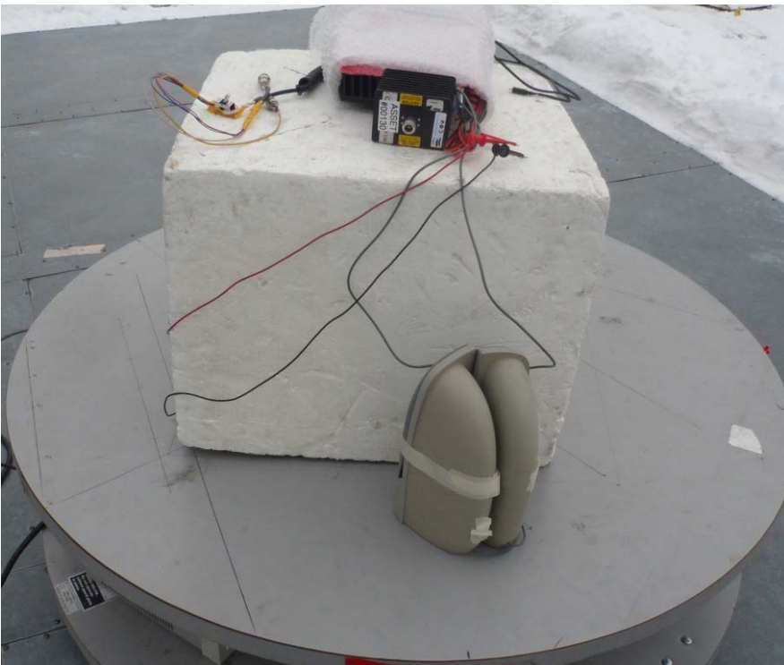
Figure E20.6 – Setup Photo – Radiated Measurements
