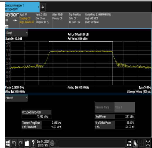
Band41(2535-2655)-15MHz-16QAM-40590-75RB#0-PASS
