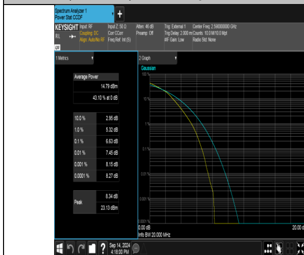
Band41(2535-2655)-20MHz-16QAM-40590-100RB#0-PASS
