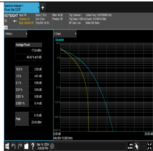
Band41(2535-2655)-15MHz-QPSK-41165-75RB#0-PASS
