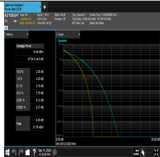
Band41(2535-2655)-20MHz-QPSK-40140-100RB#0-PASS
