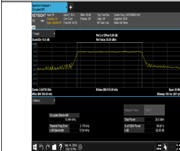
Band41(2535-2655)-15MHz-QPSK-41165-75RB#0-PASS
