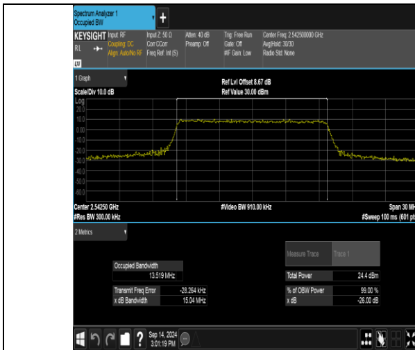
Band41(2535-2655)-15MHz-QPSK-40115-75RB#0-PASS
