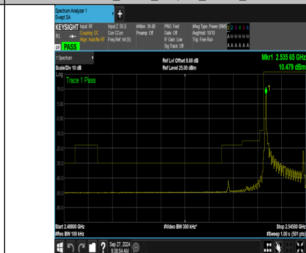
Band41_10MHz_16QAM_40090_1RB#0
