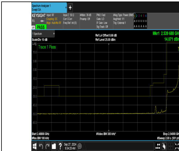
Band41_5MHz_QPSK_40065_1RB#24
