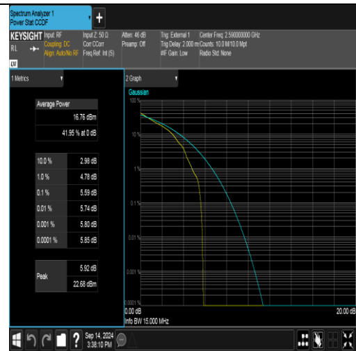
Band41(2535-2655)-15MHz-QPSK-40590-1RB#0-PASS
