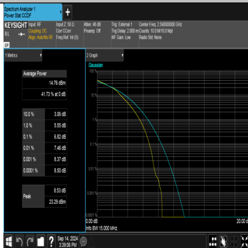
Band41(2535-2655)-15MHz-16QAM-40590-75RB#0-PASS
