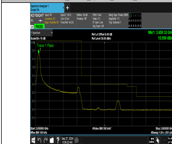
Band41_5MHz_QPSK_41215_1RB#0
