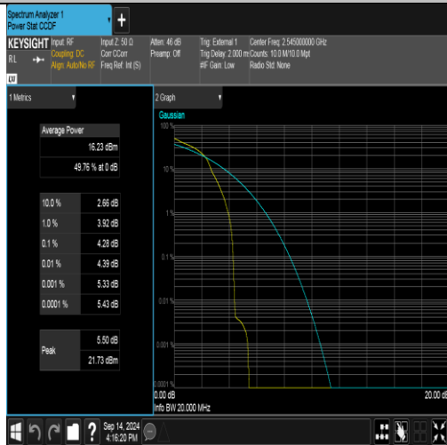
Band41(2535-2655)-20MHz-16QAM-40140-1RB#0-PASS
