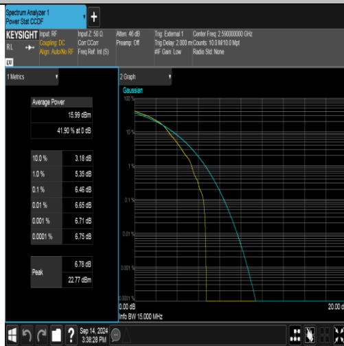
Band41(2535-2655)-15MHz-16QAM-40590-1RB#0-PASS
