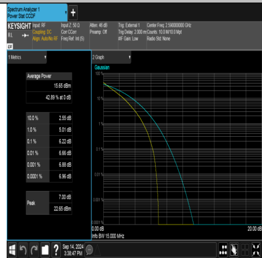
Band41(2535-2655)-15MHz-QPSK-40590-75RB#0-PASS
