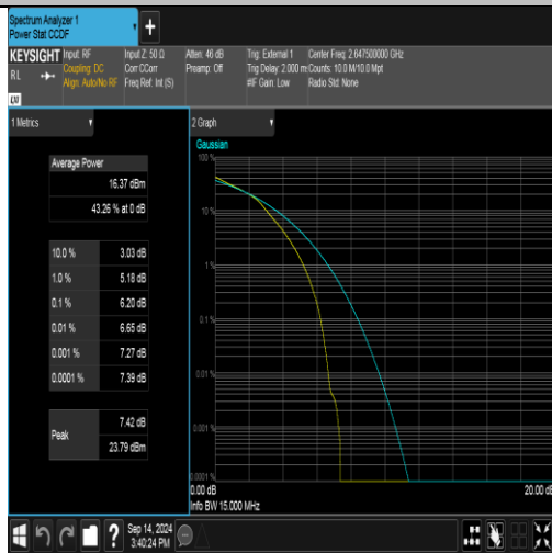
Band41(2535-2655)-15MHz-16QAM-41165-75RB#0-PASS
