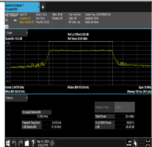
Band41(2535-2655)-15MHz-16QAM-41165-75RB#0-PASS
