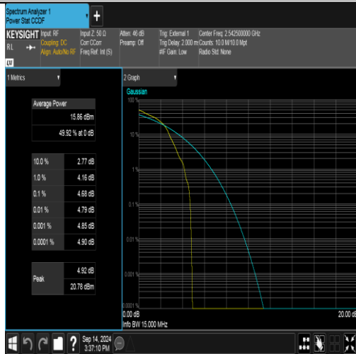
Band41(2535-2655)-15MHz-16QAM-40115-1RB#0-PASS
