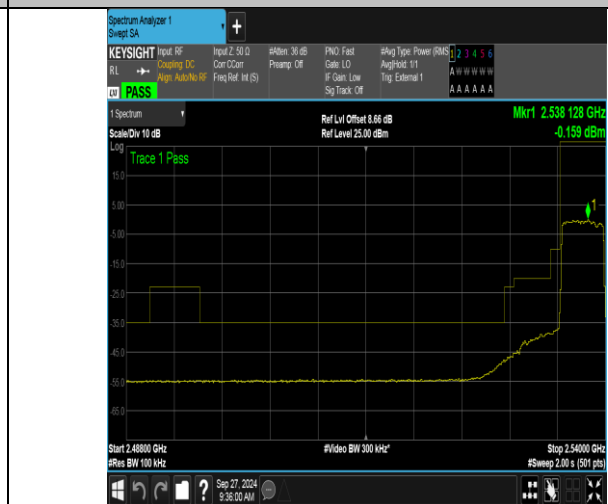
Band41_5MHz_16QAM_40065_25RB#0
