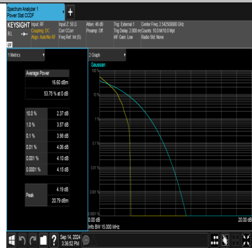
Band41(2535-2655)-15MHz-QPSK-40115-1RB#0-PASS
