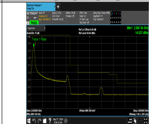
Band41_5MHz_16QAM_41215_1RB#0
