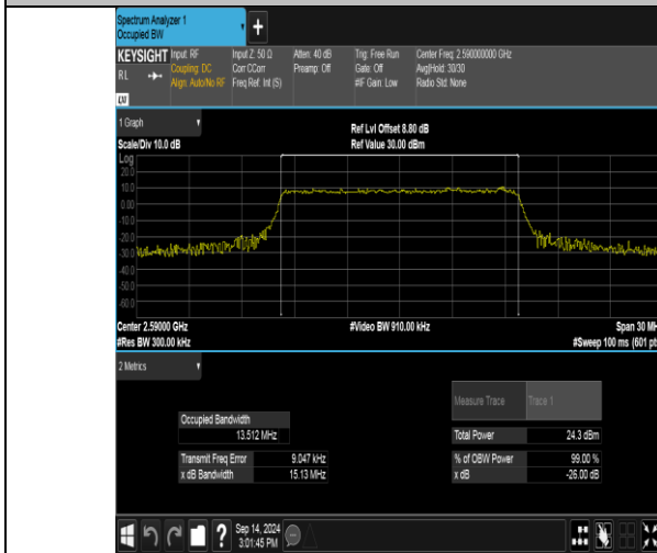
Band41(2535-2655)-15MHz-QPSK-40590-75RB#0-PASS
