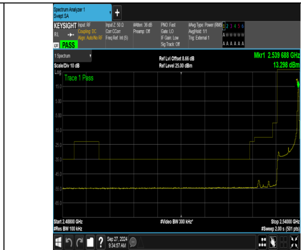
Band41_5MHz_16QAM_40065_1RB#24
