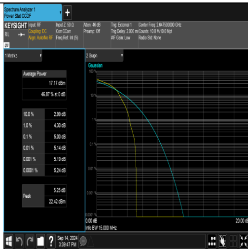
Band41(2535-2655)-15MHz-16QAM-41165-1RB#0-PASS
