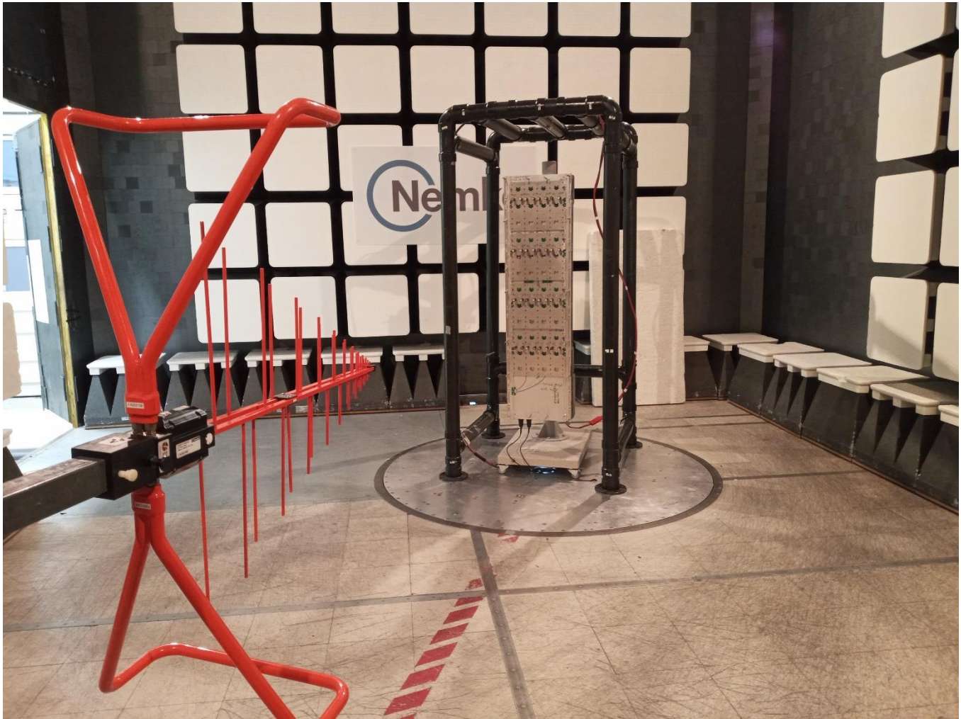
Figure 3.5-2: EUT Set-up for Radiated Compliance Testing
