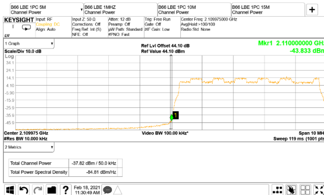
Figure 8.2-49: Conducted band edge emission at 2110 MHz, 5 MHz channel single-carrier operation (RBW = 1% of EBW)
