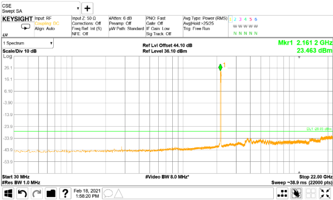
Figure 8.2-48: Conducted spurious emissions of 20 MHz two top channels, LTE + NR operation
