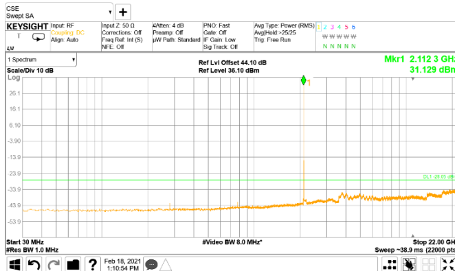
Figure 8.2-1: Conducted spurious emissions of 5 MHz low channel, single carrier operation
