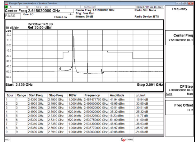
Band41_30MHz_DFT_s_OFDM_SCS30kHz_BPSK_RB1_0_CH503004
