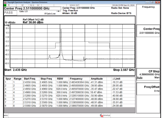
Band41_30MHz_DFT_s_OFDM_SCS30kHz_BPSK_RB1_0_CH503004
