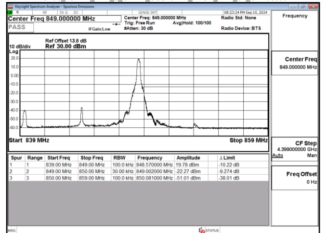
Band5 10MHz DFT_s_OFDM_SCS15kHz_BPSK_RB1_51_CH168800
