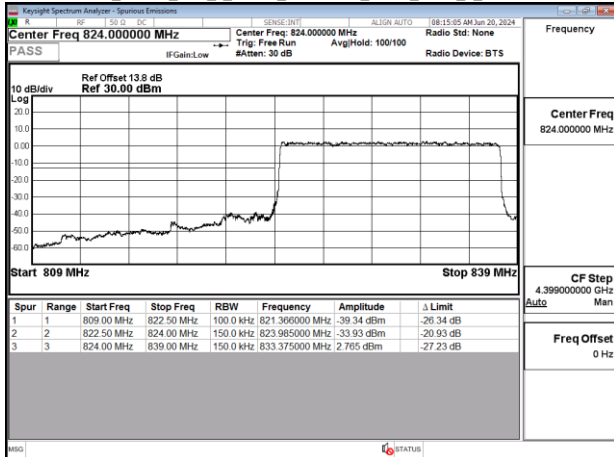
Band5_15MHz_DFT_s_OFDM_SCS15kHz_BPSK_RB75_0_CH166300
