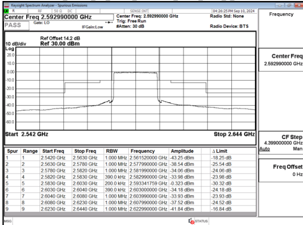
Band41_20MHz_CP_OFDM_SCS30kHz_QPSK_RB51_0_CH518598
