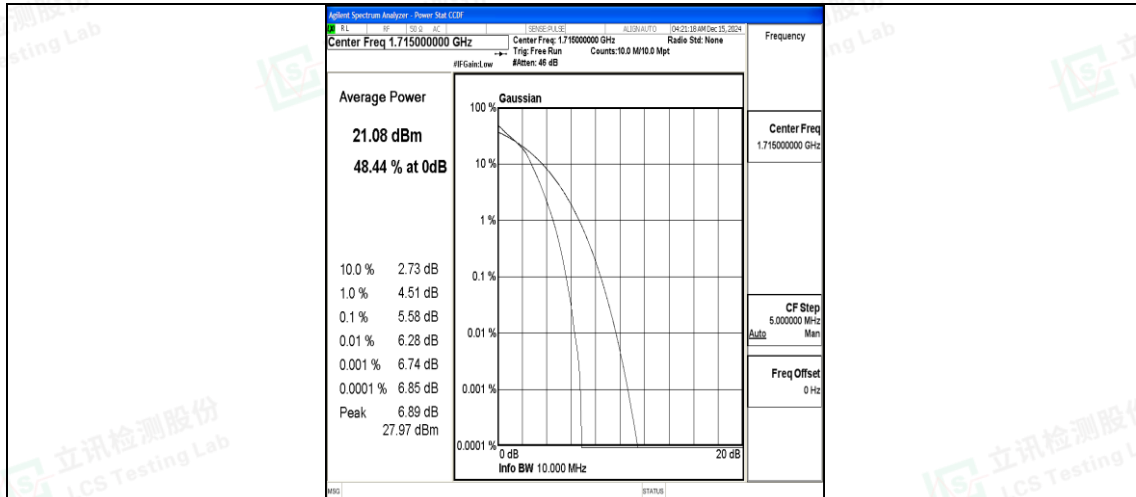
Band66-10MHz-16QAM-132022-50RB#0-PASS
