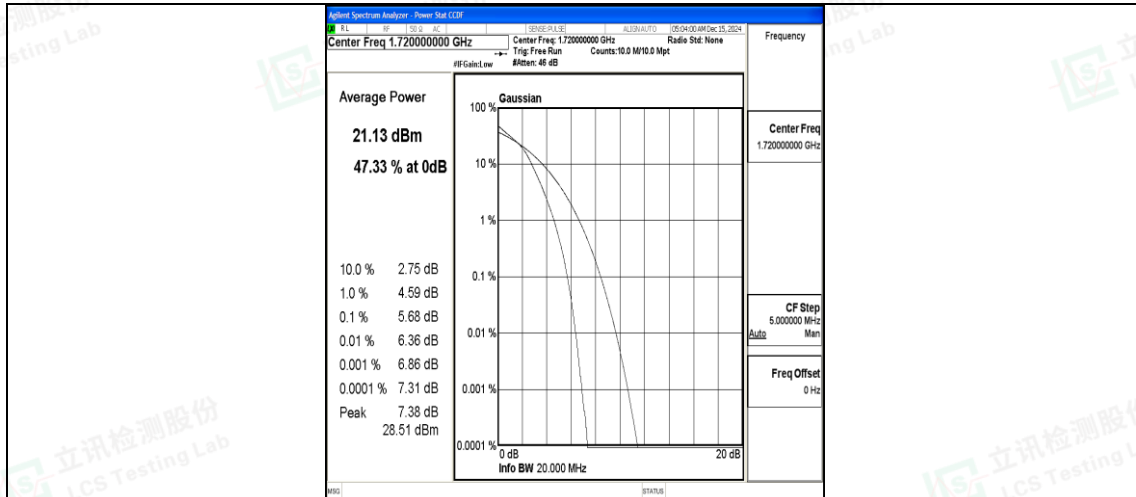
Band66-20MHz-16QAM-132072-100RB#0-PASS
