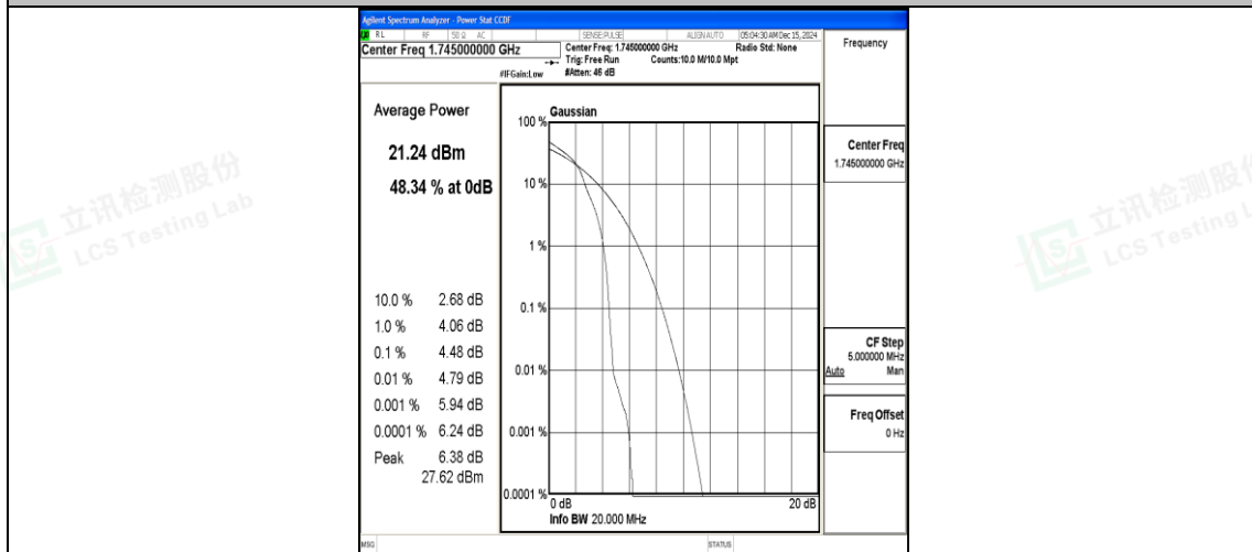
Band66-20MHz-16QAM-132322-1RB#0-PASS
