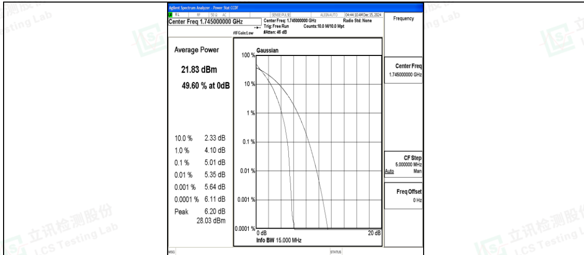
Band66-15MHz-QPSK-132322-75RB#0-PASS
