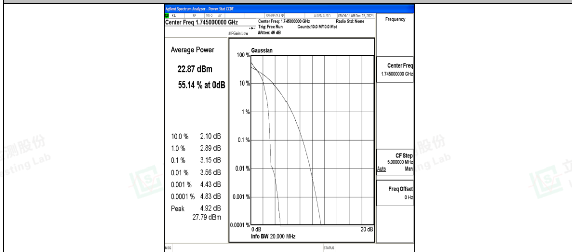
Band66-20MHz-QPSK-132322-1RB#0-PASS
