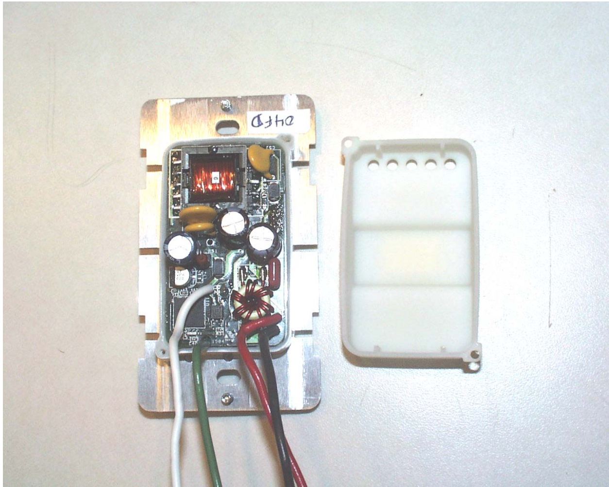
Photograph 7 - View of Side A of the Host Card
