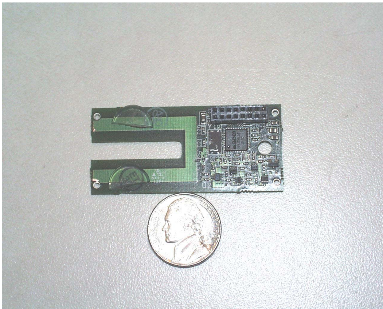
Photograph 9 - View of the Component Side of the Transceiver Card
