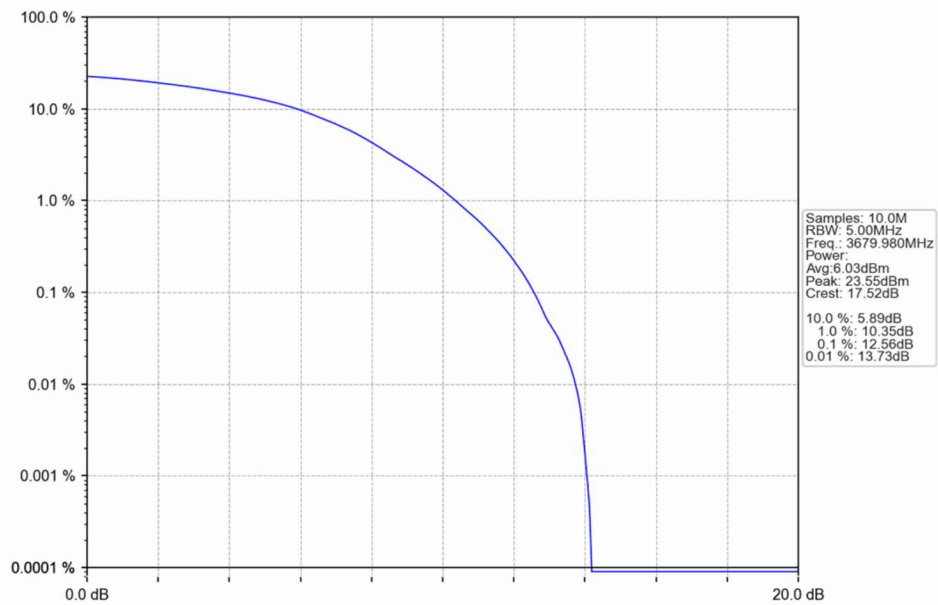
n48_30kHz_SISO_NTNV_40MHz_DFT-s-OFDM 256 QAM_3679.98MHz_Outer_Full
