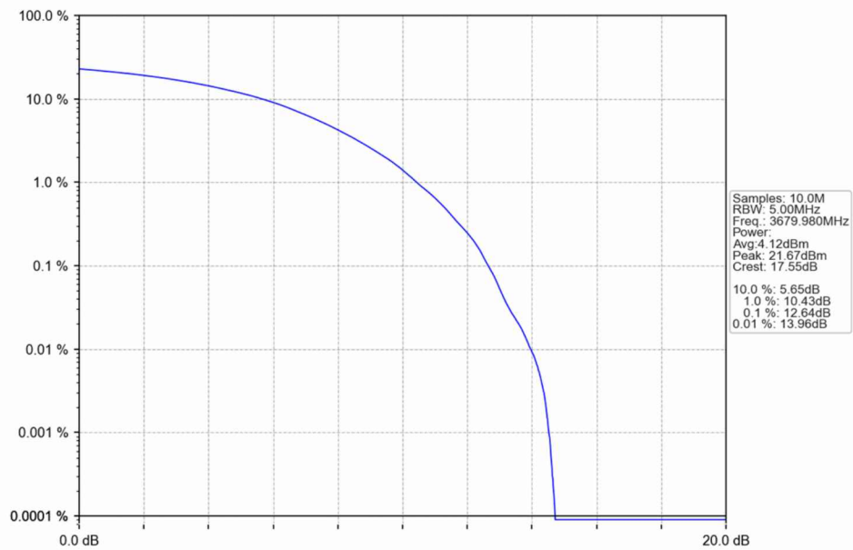
n48_30kHz_SISO_NTNV_40MHz_CP-OFDM 256 QAM_3679.98MHz_Outer_Full
