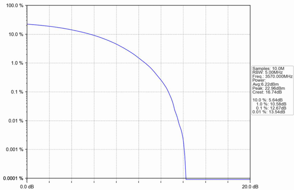
n48_30kHz_SISO_NTNV_40MHz_CP-OFDM 16 QAM_3570MHz_Outer_Full
