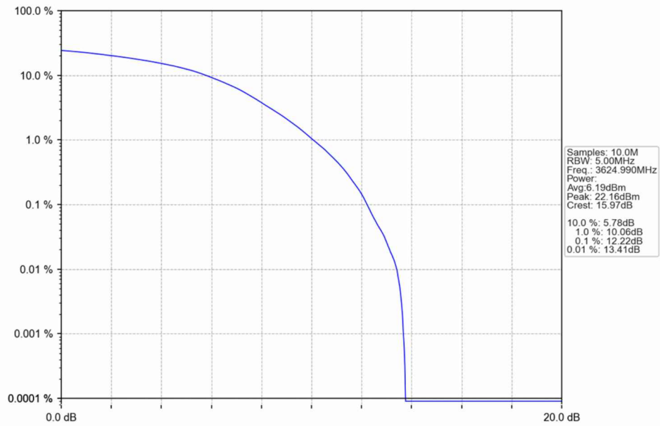
n48_30kHz_SISO_NTNV_40MHz_DFT-s-OFDM 256 QAM_3624.99MHz_Outer_Full
