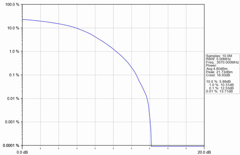
n48_30kHz_SISO_NTNV_40MHz_DFT-s-OFDM 256 QAM_3570MHz_Outer_Full
