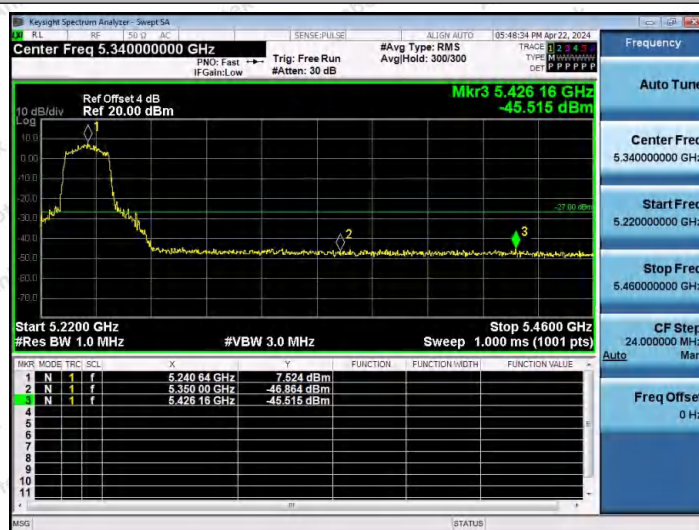
11AX20MIMO-Ant1-5240-PASS
