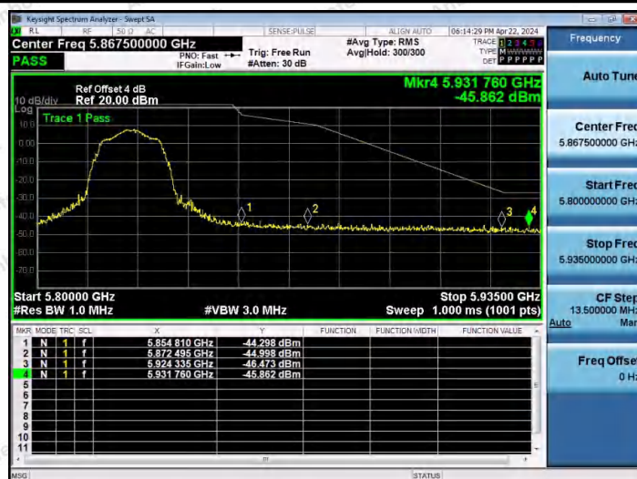
11A-Ant2-5825-PASS
