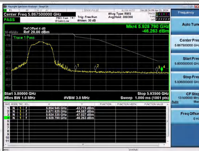
11N20MIMO-Ant2-5825-PASS
