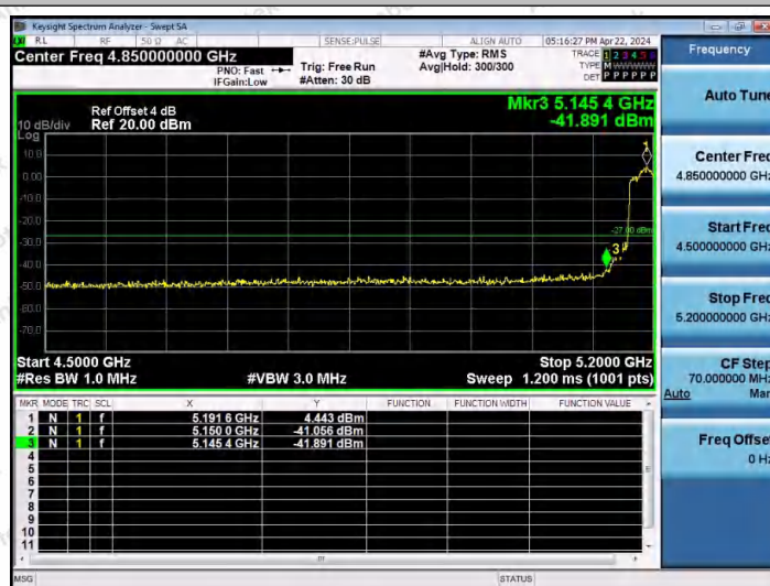
11N40MIMO-Ant1-5190-PASS
