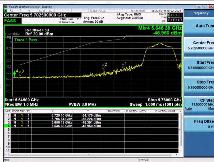
11N20MIMO-Ant2-5745-PASS
