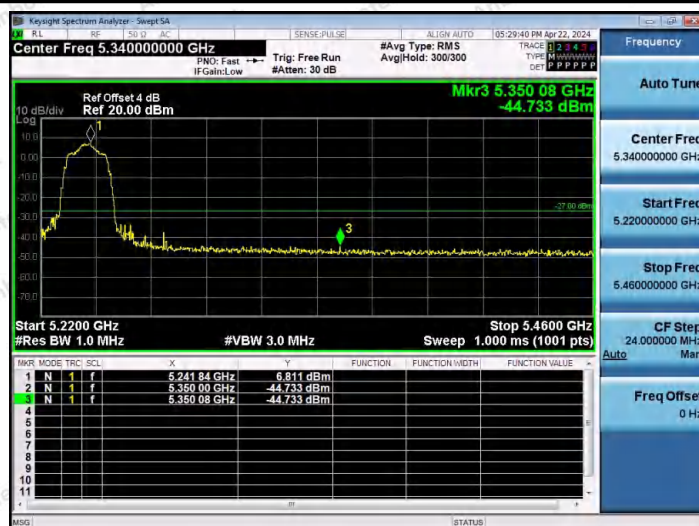
11AC20MIMO-Ant2-5240-PASS
