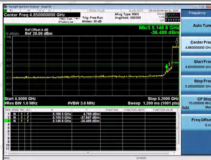
11AX40MIMO-Ant2-5190-PASS
