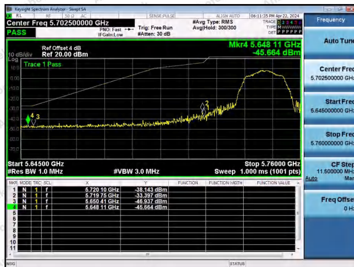
11A-Ant2-5745-PASS
