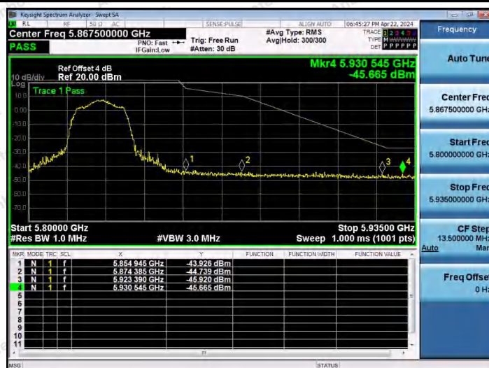
11AC20MIMO-Ant2-5825-PASS
