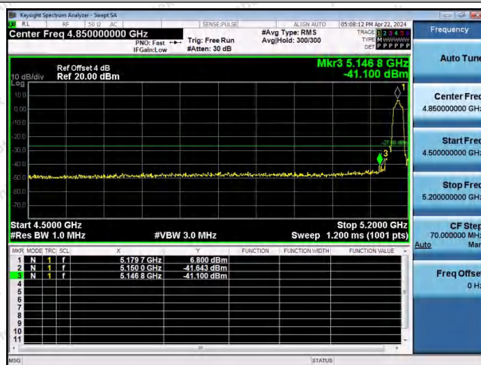
11N20MIMO-Ant2-5180-PASS
