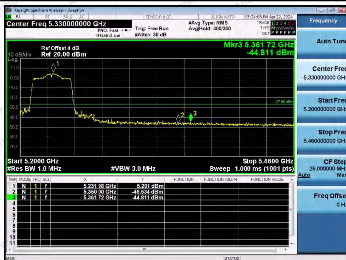
11AC40MIMO-Ant1-5230-PASS
