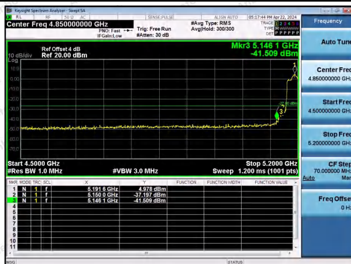
11N40MIMO-Ant2-5190-PASS
