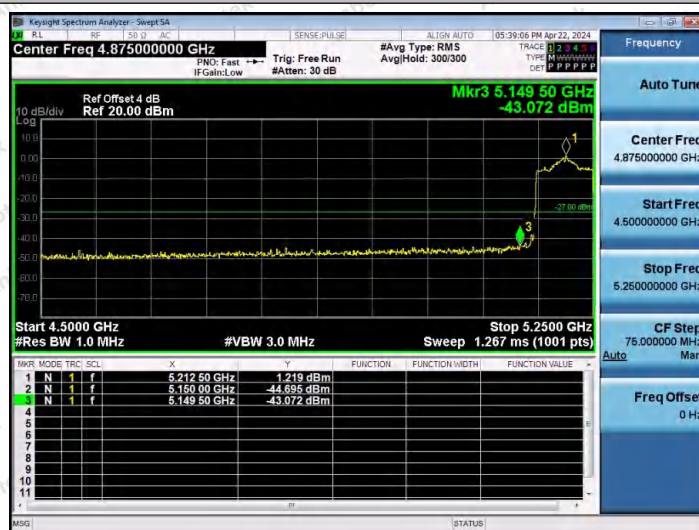
11AC80MIMO-Ant1-5210-PASS
