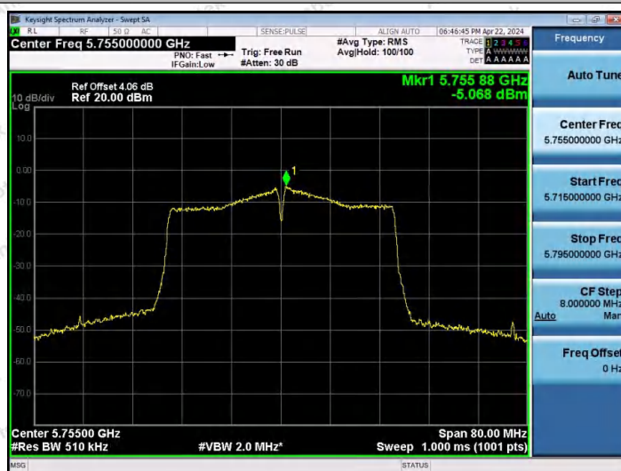
11AC40MIMO-Ant1-5755-PASS
