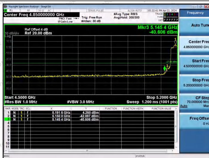
11AC40MIMO-Ant2-5190-PASS
