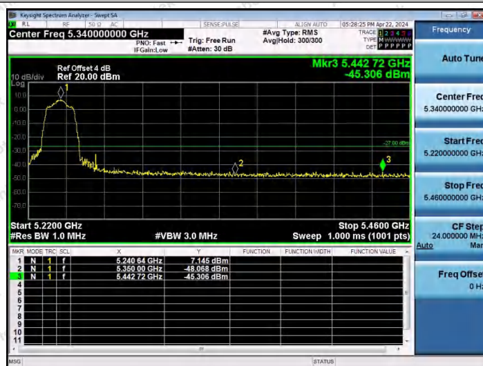
11AC20MIMO-Ant1-5240-PASS
