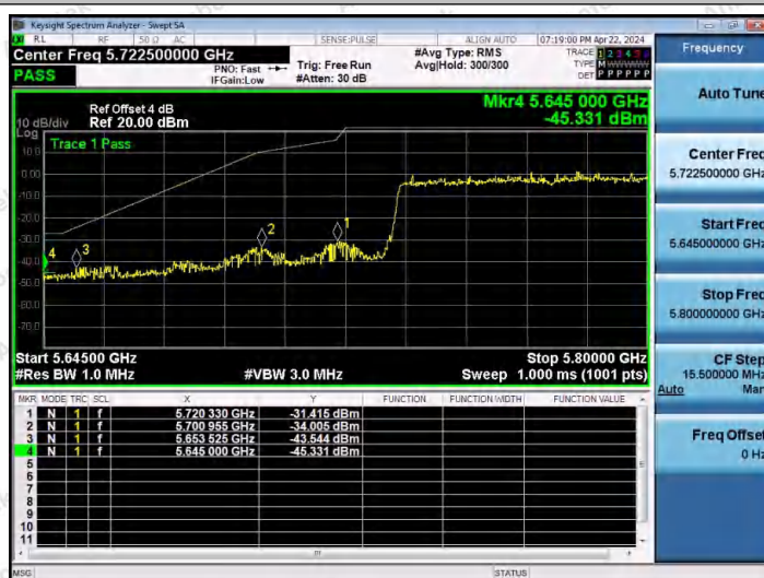
11AX80MIMO-Ant2-5775-PASS
