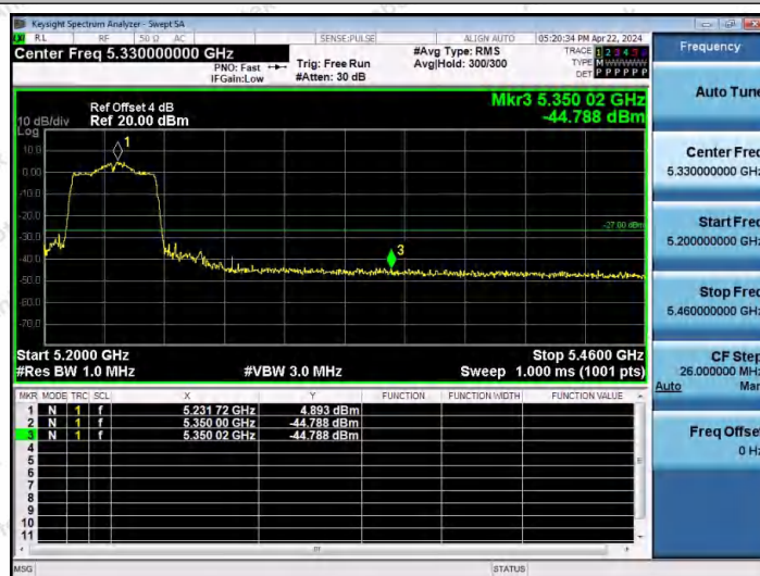
11N40MIMO-Ant2-5230-PASS
