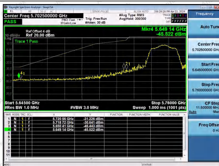
11AC20MIMO-Ant2-5745-PASS
