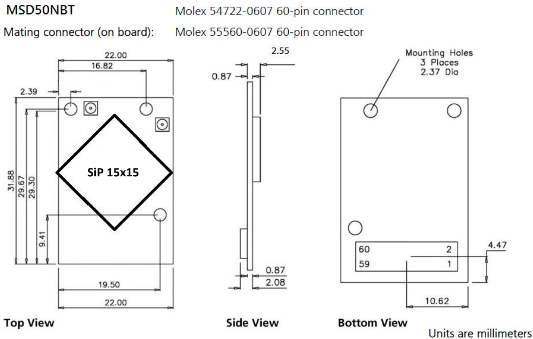
Figure 4: Module dimension of SSD50NBT
