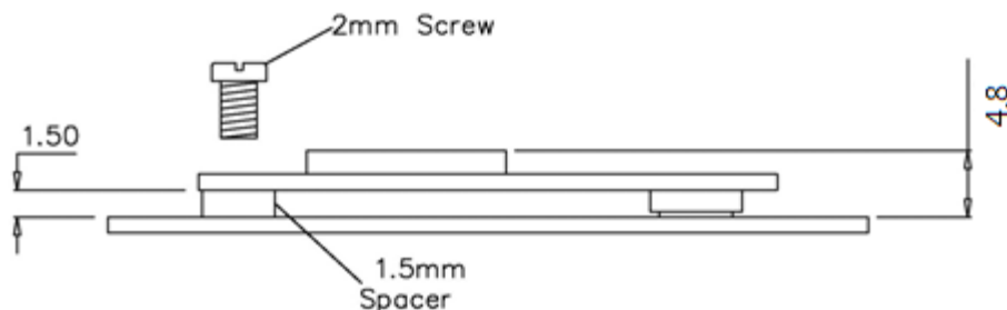
Figure 7: Mounting information for MSD50NBT
