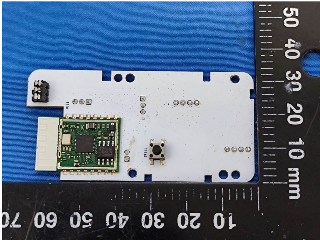
WiFi & Buletooth Antenna
