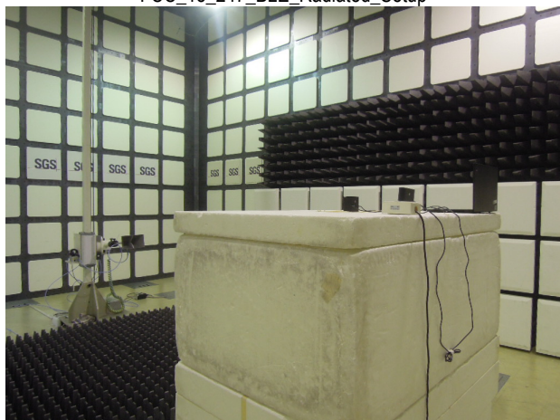
FCC_15_247_BLE_Radiated_Setup
