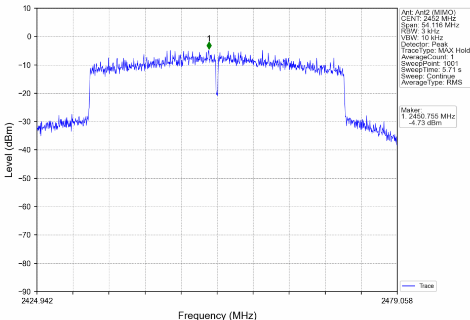
802.11ax(HEW40)_HCH_2452MHz_RU484_Left_MIMO_NTNV
