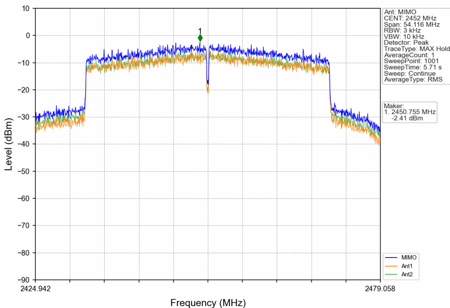
802.11ax(HEW40)_HCH_2452MHz_RU484_Left_MIMO_NTNV
