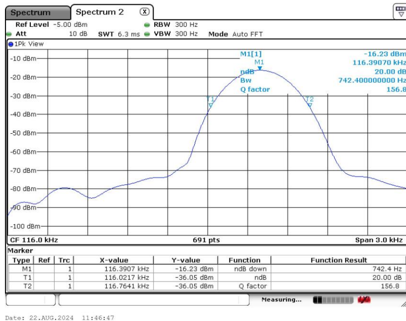
20 dB Bandwidth Plot
