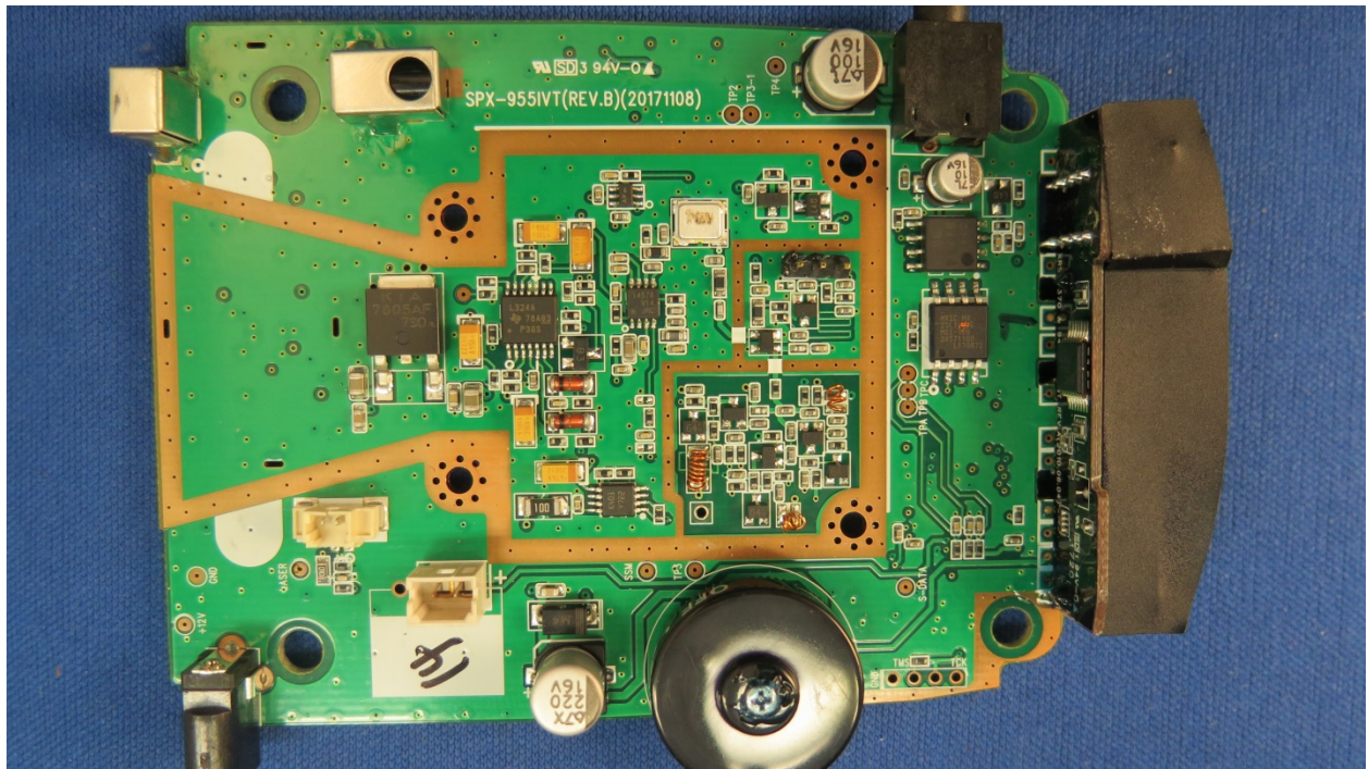
Top View – PCB Horn Removed
