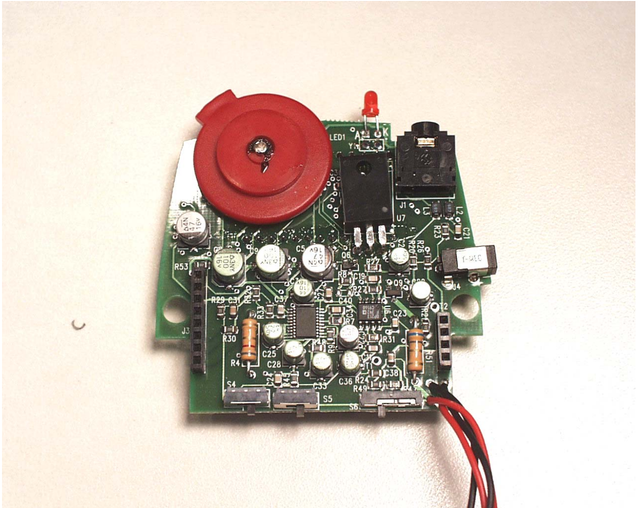
Rear Side of the Control PCB
