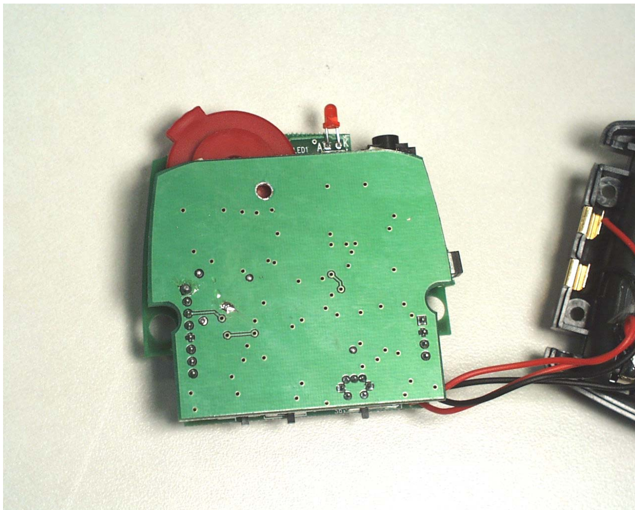
Trace Side of the Transmitter PCB While Connected to the Control Card
