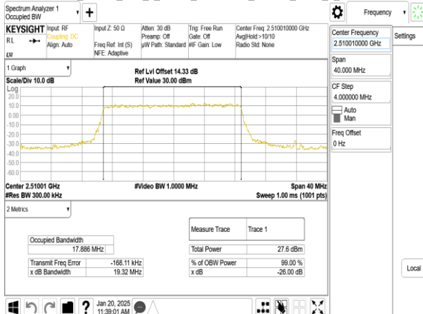
Band41_20MHz_DFT_s_OFDM_SCS30kHz_64QAM_RB50_0_CH502002
