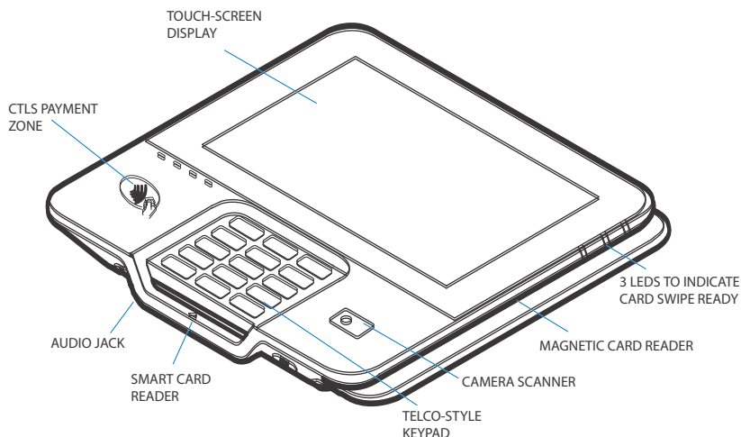
Figure 2 M424 Features
