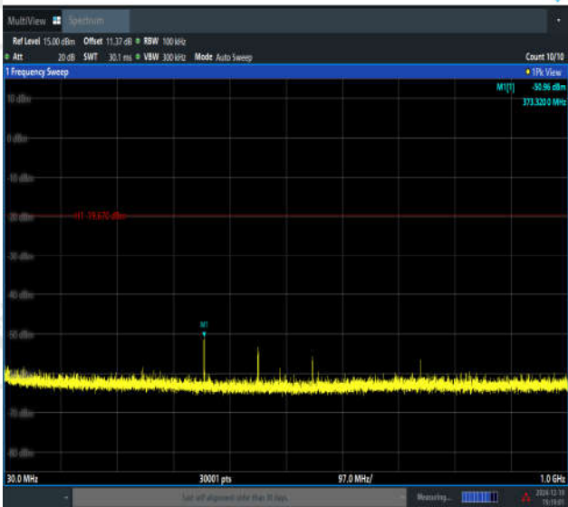
BLE_1M-Ant1-2480-30~1000-PASS
